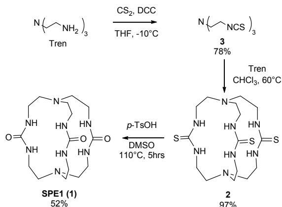
Scheme 1. Synthesis of SPE1 .
