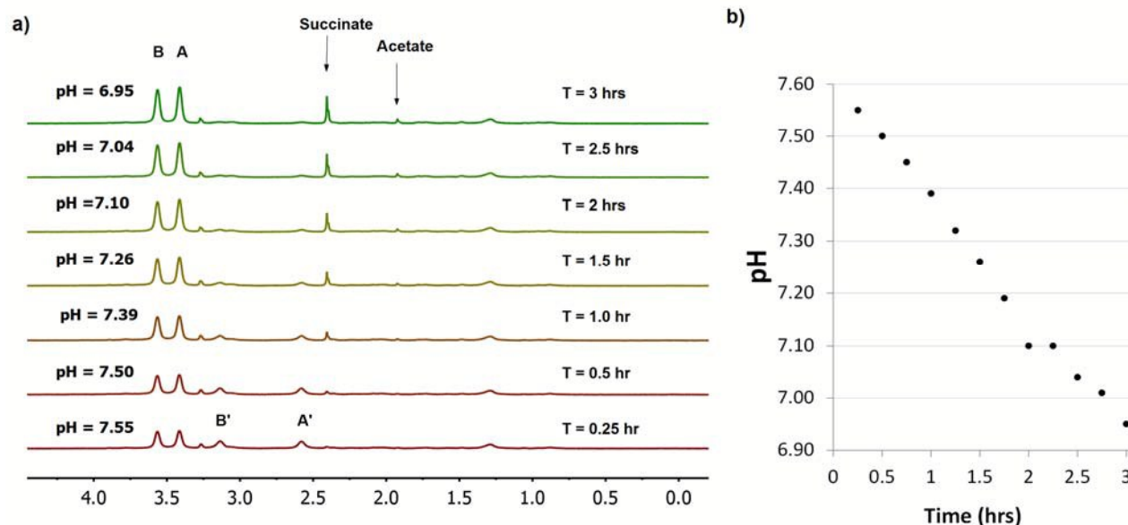
Fig. 4. Monitoring of pH in E. coli ( OD_{600} = 1 ) using 1.8 mM solution of SPE1 in phosphate buffer. a, Selected stacked ^1\text{H} NMR spectra of E. coli cells at 500 MHz in the presence of 1.8 mM SPE1 . NMR measurements were taken continuously for 3 hrs using 256 scans (15 min per experiment). b, Graph of decrease of pH overtime of SPE1 treated E. coli cells.
