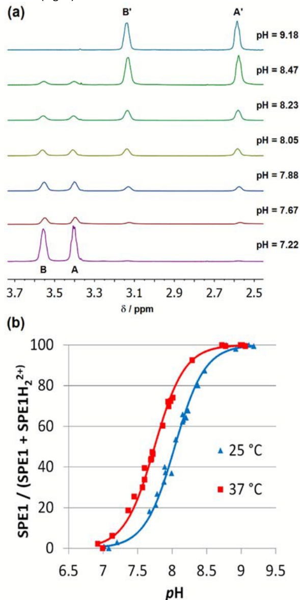
Fig. 2. 1 H NMR pH titration of SPE1 at 25 and 37 °C in phosphate buffer at 500 MHz. a, Selected partial 1 H NMR spectra of SPE1 at different pH values at 25 °C. Chemical shifts: A: 3.40 ppm, B: 3.56 ppm, A': 2.58 ppm, B': 3.13 ppm. b, Ratiometric curve of 1 H NMR pH titrations derived from the ratio of the different protonation states of SPE1 .
