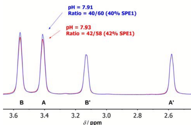
Fig. 3. Selected ^1\text{H} NMR spectra at 500 MHz showing the high accuracy of pH measurement by SPE1 . Overlay of local ^1\text{H} NMR spectra of SPE1 at pH 7.91 (blue) and 7.93 (red). The peak intensity was normalized to the signals of neutral SPE1 at 2.58 and 3.13 ppm. A difference in pH of 0.02 pH units can be detected.
