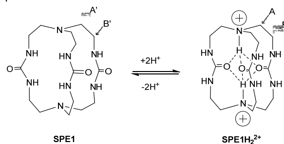
Fig. 1. Structure and protonation states of cage-shaped pH sensor SPE1 . The protons attached to the bridgehead nitrogen atoms are trapped inside the cage due to hydrogen bonding with the ureido oxygen atoms, thereby allowing SPE between two states. The 1 H NMR signals of the labelled methylene positions are used for pH sensing.
