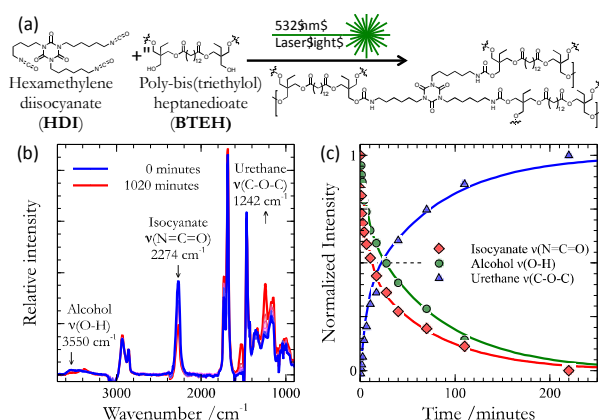
Figure 1. (a) The reaction between HDI and BTEH to form polyurethane can be followed using (b) infrared spectroscopy. In particular, formation of the urethane moiety results in the loss of bands associated with the isocyanate ( 2274\text{ cm}^{-1} ) and alcohol ( 3550\text{ cm}^{-1} ) modes, and the appearance of the C—O—C band ( 1242\text{ cm}^{-1} ) associated with the urethane. (c) The kinetics associated with these changes indicate direct conversion of isocyanates and alcohols to urethane.
