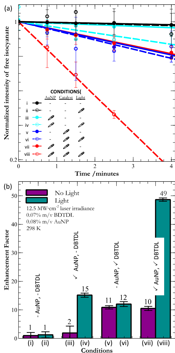
Figure 2. (a) Kinetic traces following the disappearance of the isocyanate band (2274 cm -1 ), and (b) the relative rates of reaction (with respect to pure polymer) under all eight conditions.
