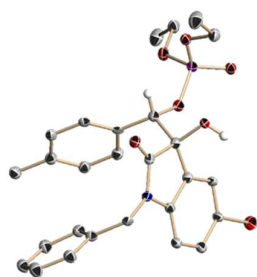
Figure 2. ORTEP diagram of 4j (Ellipsoids displayed at 50% probability. Calculated hydrogen atoms except for that attached to the stereogenic carbon atom are omitted for clarity. Black: carbon, Red: oxygen, Purple: phosphorous, Blue: nitrogen, Vermilion: bromine, White: hydrogen).
