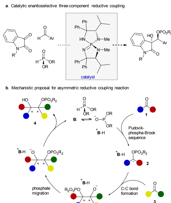
Figure 1. Stereoselective Reductive Coupling Reactions.
