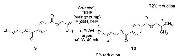
Scheme 2. Hydrogenation of the diene 9.
