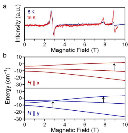
Fig. 4. a. Variable-temperature EPR spectra of 1 at 326.4 GHz applied microwave frequency. The intensities are normalized to that of the 3 T resonance. b. Zeeman energy diagrams for the M_S = 0, \pm 1 levels with the applied dc field aligned with the x - and y -axes. Solid black arrows indicate the parentage of the observed resonances in a . Full Zeeman diagrams are in Fig. S6.
