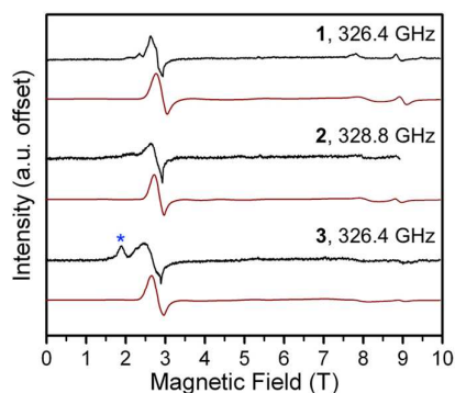
Fig. 2. Select high-frequency, high-field EPR spectra for 1–3 at 5 K. Black lines correspond to experimental data collected at the frequencies listed on the graph. Red lines are simulations with parameters given in the main text and Table 2. The blue asterisk in the spectrum of 3 indicates a peak attributed to an impurity.
