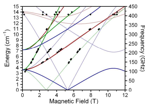
Fig. 3. Resonance field vs. microwave frequency for 1 constructed from data ( \blacklozenge ) obtained at 5 K. Solid lines represent fits to the data, with parameters as given in Table 2. Red, green, and blue lines represent x -, y -, and z -transitions, respectively. Bold lines represent ground-state M_S = 0 \rightarrow M_S = \pm 1 transitions. 21 Faded lines depict excited state transitions; those stemming from ca. 3.6 \text{cm}^{-1} correspond to excitations within the M_S = \pm 1 doublet. Excited state transitions are shown if they correspond to observed signals. See ESI for discussion of z -transitions (blue).
