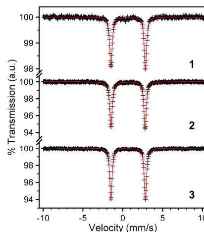
Fig. 5. Mössbauer spectra for powder samples of 1-3 collected at 80 K. Black crosses represent experimental data while red lines represent the best fits to the spectra. The parameters for these fits are given in Table 2.
