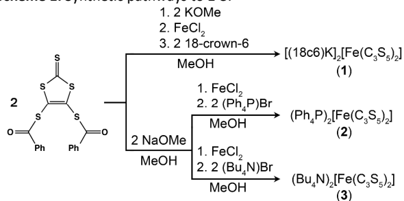
Scheme 1. Synthetic pathways to 1-3 .
