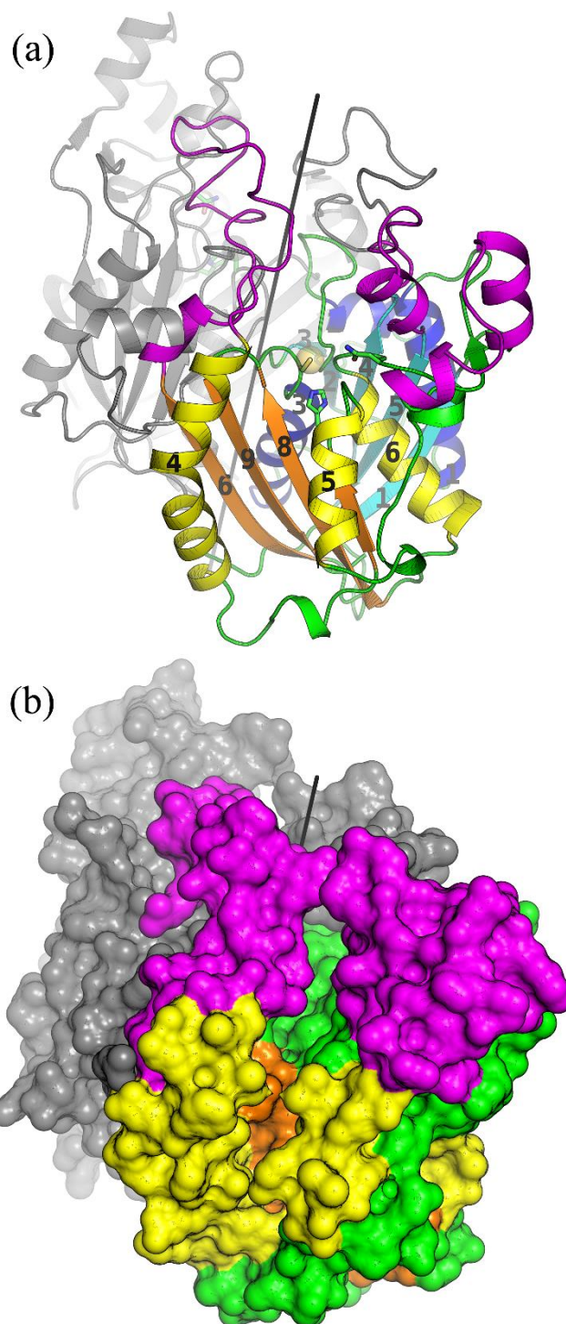
Fig. 4 Overall structure of the dimeric CorB enzyme reveals a classical thiolase fold. Both characteristic \beta\alpha\beta\alpha(\beta)\alpha\beta\beta motifs of this superfamily are coloured by their secondary structural elements in cyan and blue for the N-terminal motif and orange and yellow for the C-terminal motif. The regions exhibiting larger deviations to structural homologue enzymes are coloured in pink. The catalytic triad is represented as ball and sticks and the reactive sulfur atom of C121 is emphasized by a yellow sphere. The dimeric two-fold axis (parallel to the crystallographic two-fold axis) is shown in black. (b) Surface representation revealing a wide T-shaped active site cavity of CorB.
