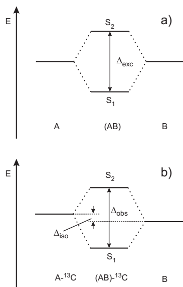
Fig. 2 Schematic view of (a) the excitonic splitting in a symmetric dimer consisting of identical chromophores A and B , (b) the S_1/S_2 state splitting in a symmetry-broken dimer that is isotopically substituted in chromophore A .
