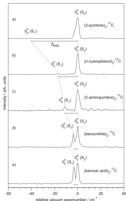
Fig. 3 Experimentally observed splittings \Delta_{obs} between the S_1 and S_2 electronic origins of the ^{13}C -isotopomers of the doubly H-bonded dimers in Figure 1.
