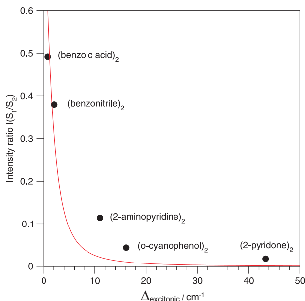
Fig. 5 Dependence of the S_1/S_2 intensity ratio on the excitonic splitting in H-bonded symmetric molecular dimers. The excitonic splittings were observed from the directly observable splittings of the ^{13}\text{C} isotopomers, assuming a ^{12}\text{C}/^{13}\text{C} isotopic shift \Delta_{iso} of 3.3 \text{ cm}^{-1} for all dimers. The theoretical dependence of the S_1/S_2 intensity ratio on \Delta_{exc} is indicated in red.
