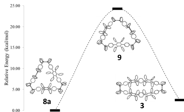
Fig. 4. Comparison of strain energies of 8a , 9 , and 3 , using DFT calculations at the B3LYP/6-31G(d) level of theory. For all structures, methoxy groups are substituted by hydrogen atoms. Hydrogen atoms are omitted for clarity.
