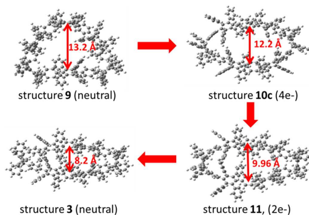
Fig. 5. Geometric analysis of structures 9 , 10c , 11 and 3 to understand the equilibrium structure of tetraanion 10c , using DFT calculations at the B3LYP/6-31G(d) level of theory. Structure 11 is twice negatively at one cyclohexadiene moiety, whereas the other contains contains to hydrogen atoms, analogously to the other structures.
