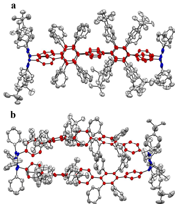
Fig. 6. Crystal structure of 3 . ORTEP drawing at 50% probability level. All hydrogen atoms are omitted for clarity. Phenylene moieties are labelled in red. 3,6-bridging cyclohexa-1,4-dienes are labelled in blue. Front view (a) and top view (b).
