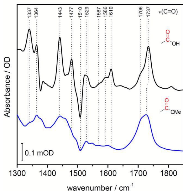
Figure 4: SEIRA spectrum of immobilized FePOH (black) and FePOMe (blue) in ACN. The SAM coated Au electrode was used as reference spectrum.
