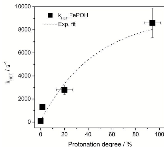
Figure 7: Protonation degree of the carboxylic acid hanging group of FePOH in % calculated via equation (1) plotted vs. the TR-SERR spectroscopic derived k_{\text{HET}} in Table 1. The dashed line represents an exponential fit to the data.
