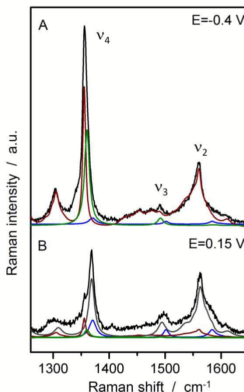
Figure 2: SERR spectra of FePOH in 100 mM PBS buffer at -0.4 V and +0.15 V vs. Ag/AgCl 3M with the respective component spectra: HS red (red), HS ox (grey), LS red (green), LS ox (blue)
