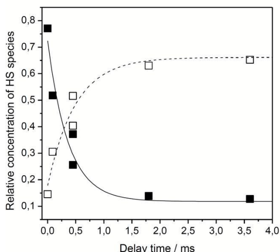
Figure 6: Relative contribution of the Fe III -HS (solid squares) and Fe II -HS (hollow squares) species of FePOH as a function of delay time after a potential jump from 0.15 V to -0.4 V.
