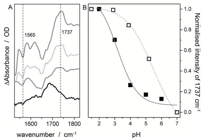
Figure 5: SEIRA difference spectrum of FePOH in PBS buffer of different pH. From bottom to top: pH= 5.5, 4.3, 3.0 and 1.6. The spectrum at pH 7 was used as reference. B: Normalized intensity of the 1737 \text{cm}^{-1} band (or the 1715 \text{cm}^{-1} band in \text{D}_2\text{O} ) as a function of pH.
