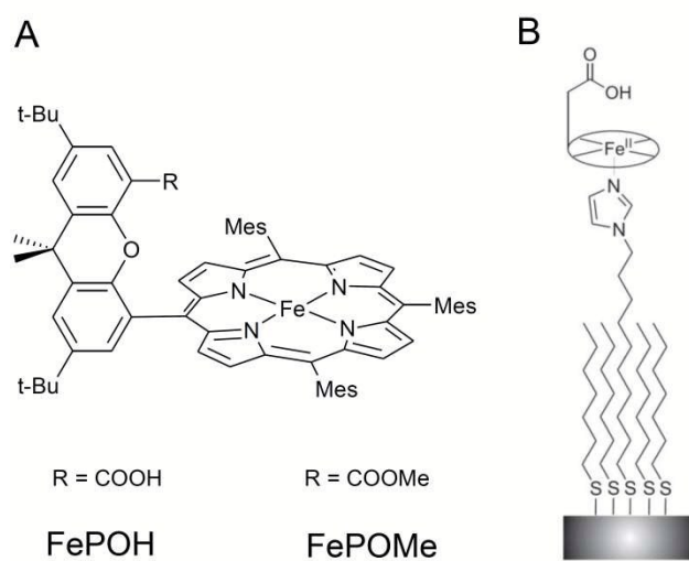
Figure 1: A: Structure of FePOH and FePOME hangman complexes. B: Schematic representation of the hangman immobilization on electrodes using a mixed imidazole terminated SAM.
