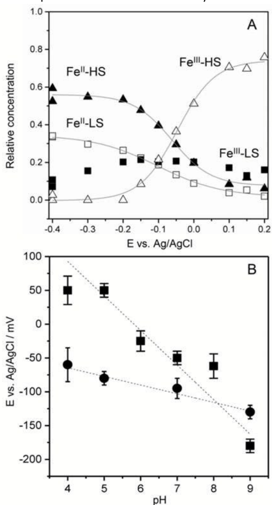
Figure 3: A: Relative contributions of the FePOH component spectra ( \text{Fe}^{\text{III}}\text{-HS} : open triangles, \text{Fe}^{\text{II}}\text{-HS} : solid triangles, \text{Fe}^{\text{III}}\text{-LS} : solid squares, \text{Fe}^{\text{II}}\text{-LS} : open squares) as a function of electrode potential. B: Redox potentials of FePOH (squares) and FePOMe (circle).
