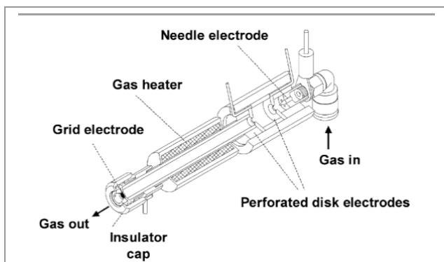
Figure 7. Cross Sectional Diagram of a DART Source. Reprinted with permission from reference 76. Copyright 2005 American Chemical Society.
