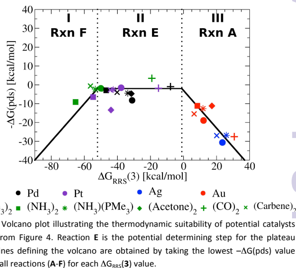
Figure 5. Volcano plot illustrating the thermodynamic suitability of potential catalysts derived from Figure 4. Reaction E is the potential determining step for the plateau region. Lines defining the volcano are obtained by taking the lowest -\Delta G(\text{pds}) value amongst all reactions (A-F) for each \Delta G_{\text{RRS}}(\mathbf{3}) value.
