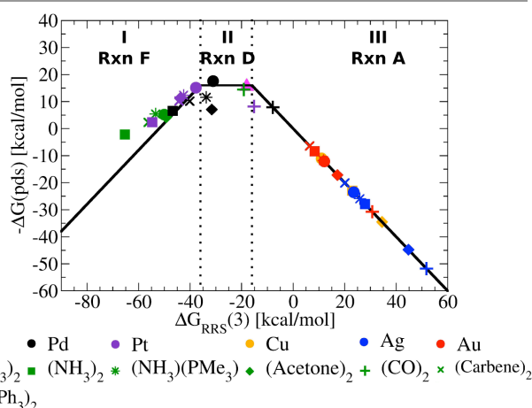
Figure 7. Refined volcano plot illustrating the thermodynamic suitability of potential catalysts where the isomerization and ligand exchange steps are ignored. The most attractive candidates lie near the top of the volcano in region II. Equations used to derive the volcano are presented in the ESI.
