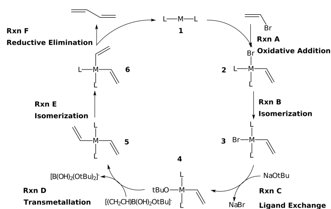
Figure 1. Reaction mechanism for the Suzuki cross-coupling of olefins.
