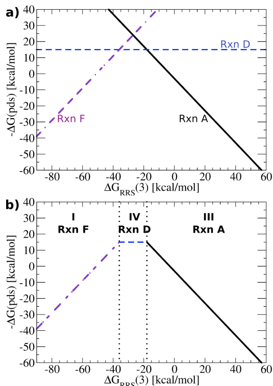
Figure 6. (a) Plot of linear scaling relationships, derived from intermediates where reactions B,C , and E have been removed because they are known to occur rapidly based on experimental observations. Reactions A (oxidative addition) and F (reductive elimination) appear as sloped lines. (b) Volcano plot derived from Figure 6a. Reaction D is the potential determining step for the plateau region. Lines defining the volcano are obtained by taking the lowest -\Delta G(\text{pds}) value amongst all reactions for each \Delta G_{\text{RRS}}(\mathbf{3}) value.
