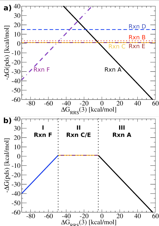
Figure 4. (a) Plot of linear scaling relationships, derived from intermediates (Reactions B-E), depicted as straight lines from the corresponding linear relationships (Figure 3). Reactions A (oxidative addition) and F (reductive elimination) appear as sloped lines. (b) Volcano plot derived from Figure 4a. Reactions C and E are the potential determining step for the plateau region. Lines defining the volcano are obtained by taking the lowest -\Delta G(\text{pds}) value amongst all reactions for each \Delta G_{\text{RRS}}(\mathbf{3}) value.
