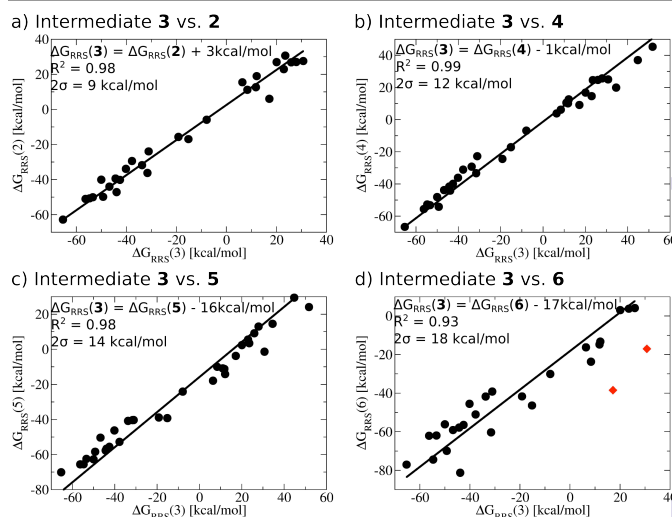
Figure 3. Linear scaling relationships amongst intermediates. Free energies ( \Delta G_{\text{RRS}} ) are relative to the catalytic resting state, as defined by Equations 2-6. Equations defining the linear scaling relationships (upper left) are used to create volcano plots (vide infra). No comparison between 1 and 3 is not possible, since \Delta G_{\text{RRS}}(\mathbf{1}) is, by definition, zero. Comparisons with 3 are equal to unity. Red points in Figure 3d have been excluded from the data fitting equations based on Grubbs' statistical test for outliers. Note that equations derived from the linear scaling relationships appear to be independent of computational level (see ESI for details).
