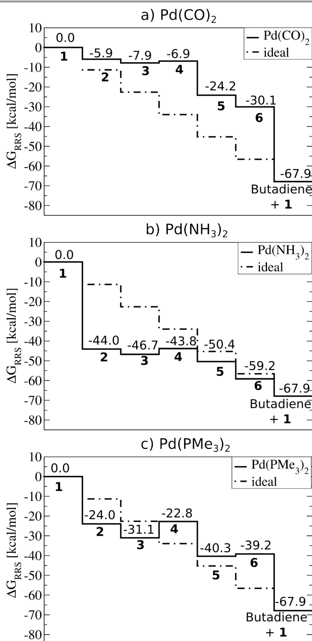
Figure 2. Free energy plots (PBE0-dDsC/TZ2P//M06/def2-SVP, COSMO-RS Solvation) relative to the resting state ( \Delta G_{RRS} , defined by Equations 2-6) for selected catalysts: (a) Pd(CO) 2 , (b) Pd(NH 3 ) 2 , (c) Pd(PMe 3 ) 2 . Moving between different species (1-6) corresponds to completing the corresponding reaction (A-F) given in Figure 1.
