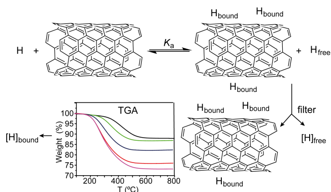
Scheme 1. Procedure for the measurement of [H]_{\text{bound}} and [H]_{\text{free}} . A known concentration of host molecule H and SWNTs are allowed to reach equilibrium, and then complex and free species are physically separated through filtration. The concentration of [H]_{\text{bound}} is measured by TGA (typical results for a titration experiment are shown, see the Supporting Information for full data set). The concentration of [H]_{\text{free}} can then be calculated by subtraction or directly measured in the filtrate.
