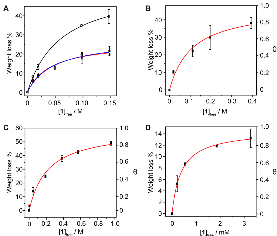
Figure 2. Titrations of pyrene vs pp-SWNTs in a) THF at 0.1 mg/mL of SWNTs (circles and black line, K_a = 16.4 \pm 0.8 \text{ M}^{-1} , r^2 = 0.999 ); 1 mg/mL of SWNTs (squares and red line, K_a = 24 \pm 6 \text{ M}^{-1} , r^2 = 0.979 ); and 10 mg/mL of SWNTs (triangles and blue line, K_a = 21 \pm 4 \text{ M}^{-1} , r^2 = 0.985 ); b) DMF ( K_a = 9 \pm 3 \text{ M}^{-1} , r^2 = 0.978 ); c) TCE ( K_a = 4.5 \pm 0.9 \text{ M}^{-1} , r^2 = 0.987 ); d) MeOH ( K_a = 2.6 \pm 0.2 \times 10^3 \text{ M}^{-1} , r^2 = 0.998 ). Each data point is the average of three separate experiments, and the error bars represent the standard deviation. Solid red lines represent the fit.
