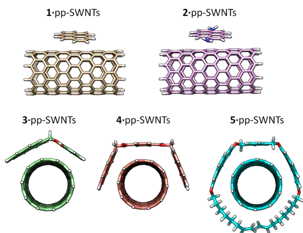
Figure 5. Minimum-energy geometry for the supramolecular assemblies formed by hosts 1-5 vs pp-SWNTs calculated at the PBE0-D3/6-31G** level of theory.
