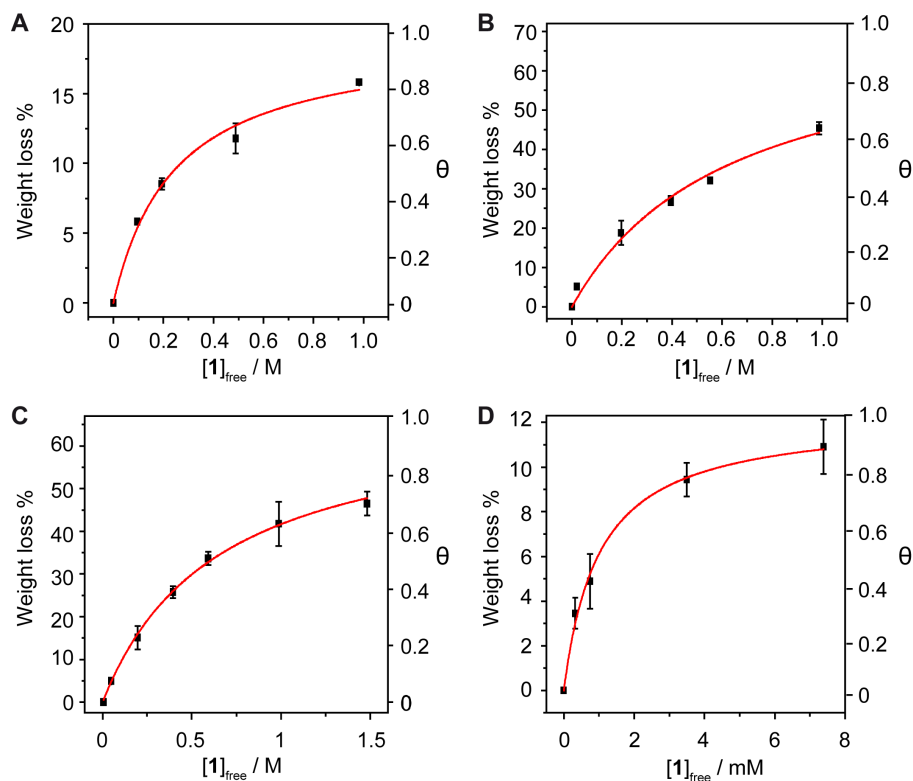
Figure 3. Titrations of 1 vs (6,5)-SWNTs in a) THF ( K_a = 41 \pm 8 \text{ M}^{-1} , r^2 = 0.987 ); b) DMF ( K_a = 1.6 \pm 0.4 \text{ M}^{-1} , r^2 = 0.985 ); c) TCE ( K_a = 1.6 \pm 0.1 \text{ M}^{-1} , r^2 = 0.998 ); d) MeOH ( K_a = 1.0 \pm 0.1 \times 10^3 \text{ M}^{-1} , r^2 = 0.994 ). Each data point is the average of three separate experiments, and the error bars represent the standard deviation. Solid red lines represent the fit.
