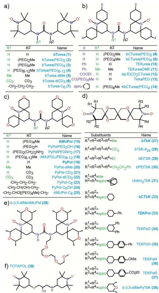
Figure 1. Structures and names of the radicals investigated in this study: (a) the bTurea series, (b) the bCTurea series, (c, e) the PyPol series, (d) the bTbK series. The TOTAPOL (f) and bCTbK (d) structures given for completeness. The prefix spiro indicates junction through just one carbon atom. PEG indicates a -\text{CH}_2\text{CH}_2\text{O}- unit. Molecular weights and synthetic routes are given in the Supplementary Information.
