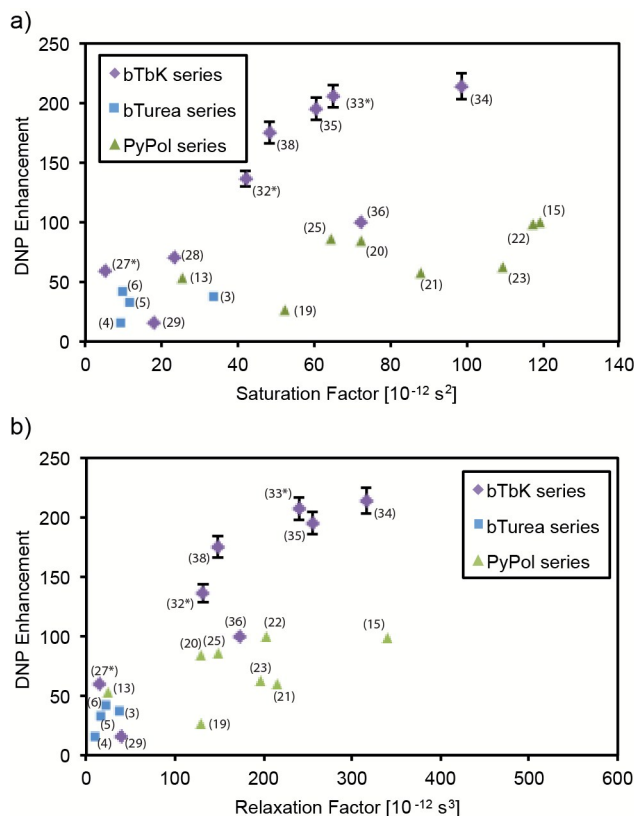
Figure 3. DNP enhancement ( \epsilon_{\text{C CP}} ) as a function of saturation factor ( T_{1e}-T_{2e} ) and relaxation factor ( T_{1e}-T_{2e}-T_{1n} ) for selected compounds from (a, b) the bTurea series (TCE, 16 mM), (c, d) the PyPol series (TCE, 16 mM), (e, f) the bTbK series (TCE, 16 mM). The data points marked with an asterisk are taken from the previous study by Zagdoun et al. 14 Error bars are shown where larger than the symbols.
