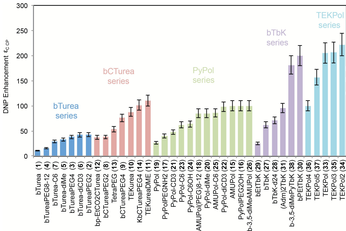
Figure 2. ^1\text{H} - ^{13}\text{C} CP DNP enhancement ( \epsilon_{\text{CCP}} ) for bulk solutions of TCE with 16 mM radical.
