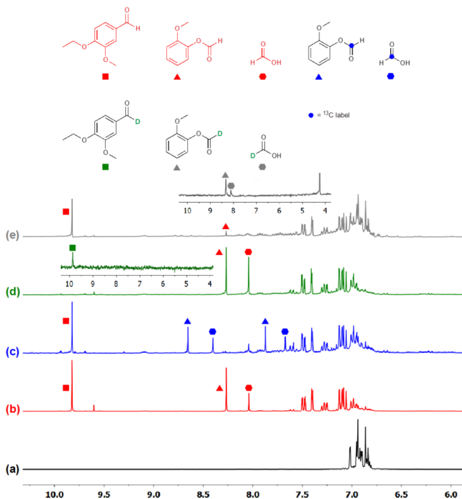
Fig. 5 NMR (300 MHz, CD_3CN ) spectra of lignin model compounds before and after photocatalytic reactions. (a) Compound 11 ; (b) 11 after photolysis; (c) 11 - ^{13}C_2 after photoreaction; (d) 11 - D1 after photoreaction (inset: ^1H -decoupled ^2H NMR spectrum of 6 - D ); and (e) 11 - D2 after photoreaction (inset: ^1H -decoupled ^2H NMR spectrum after partial conversion). The peak at 4.27 ppm is from unreacted 11 - D2 . The unlabeled products 6 (red square), 9 (red triangle), and formic acid (red hexagon) are indicated at their distinctive chemical shifts. The ^{13}C labeled 9 - ^{13}C_1 (blue triangle) and ^{13}C labeled formic acid (blue hexagon) have been split due to the ^1H coupling with ^{13}C . The deuterated 6 - D (green square), 9 - D (grey triangle), and formic acid (grey hexagon) have been detected by ^2H NMR spectroscopy.
