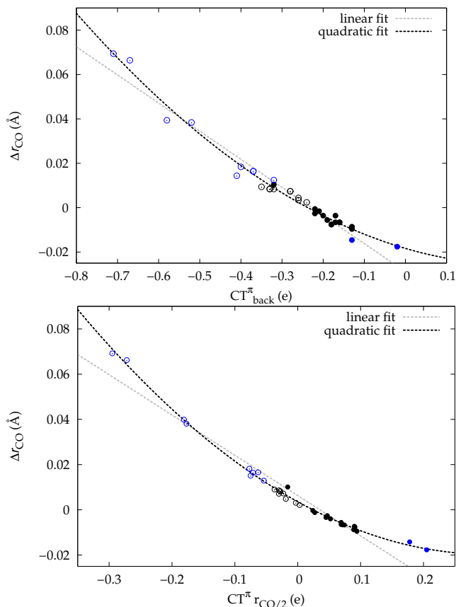
Fig. 7 Correlation between CO bond-length change upon coordination, \Delta r_{\text{CO}} , and (a) M→CO \pi back-donation \text{CT}_{\text{back}}^{\pi} (upper panel) (b) CO \pi electron polarization \text{CT}_{r_{\text{CO}/2}}^{\pi} (lower panel), for the whole set of complexes studied. Black-colored points refer to the gold(I) complexes, blue-colored points to the homoleptic carbonyls (filled circles are for positively charged complexes, empty circles for neutral or negatively charged ones). Both the linear fit ( R^2=0.959 for the upper panel, R^2=0.945 for the lower panel) and the quadratic fit ( R^2=0.984 for the upper panel and R^2=0.996 for the lower panel) curves are shown.
