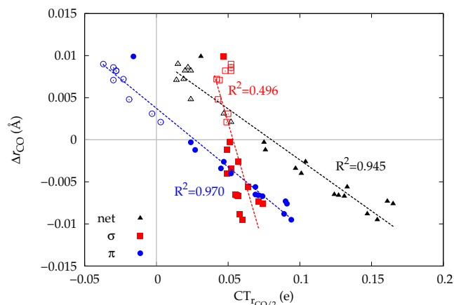
Fig. 6 Correlation between the computed \Delta r_{CO} in the considered series of [(L)Au(CO)]^{0/+} complexes and CT_{rCO/2} (black triangles), CT_{rCO/2}^{\sigma} (red squares) and CT_{rCO/2}^{\pi} (blue circles). Empty symbols are for the neutral species, filled symbols for the cationic species.
