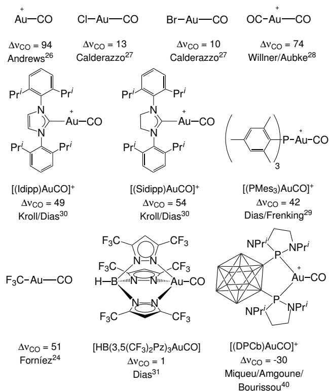
Fig. 1 The experimentally characterized gold(I) carbonyl complexes discussed in this work, with the observed carbonyl stretching frequency shifts, \Delta\nu_{CO} (in cm^{-1} ), and literature references.
