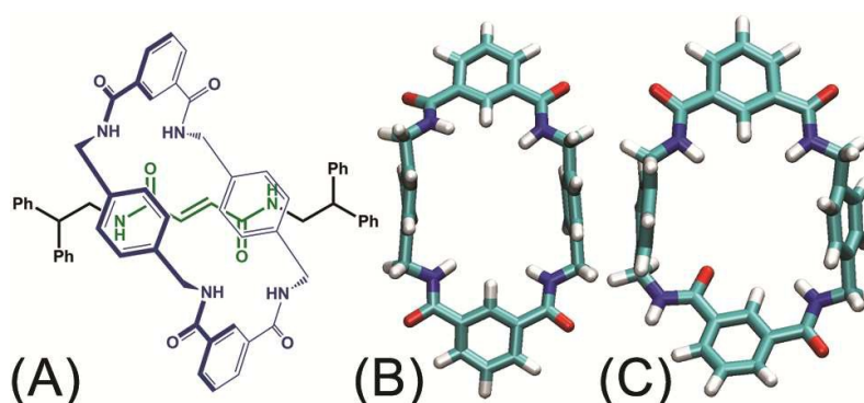
Figure 1. (A) Chemical structure of the rotaxane molecule studied in this contribution. (B) The ground state of the ring. All amide moieties adopt syn conformation. (C) The excited state of the ring. Amide moieties adopt three syn and one anti conformation.
