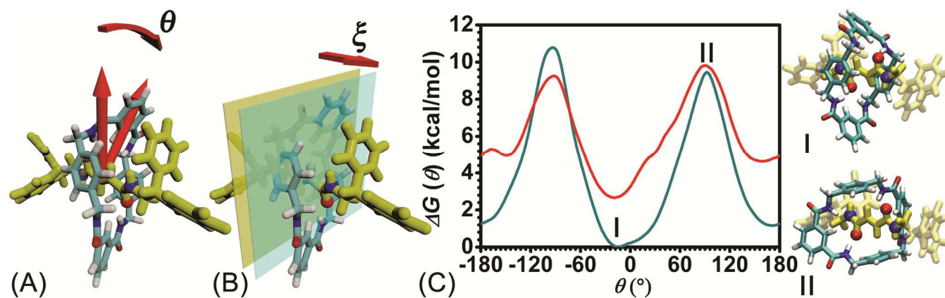
Figure 2. Definition of the collective variables — (A) \theta , characterizing the rotational angle of the ring about the thread, and (B) \zeta , the projection of the vector connecting the barycenter of the ring to the thread along the z -coordinate. (C) Free-energy profiles delineating the rotary movement of the ring in its ground (cyan curve) and excited states (red curve) about the thread along transition coordinate \theta . The three-dimensional structures of configurations I and II charted on the cyan curve are shown on the right-hand side.
