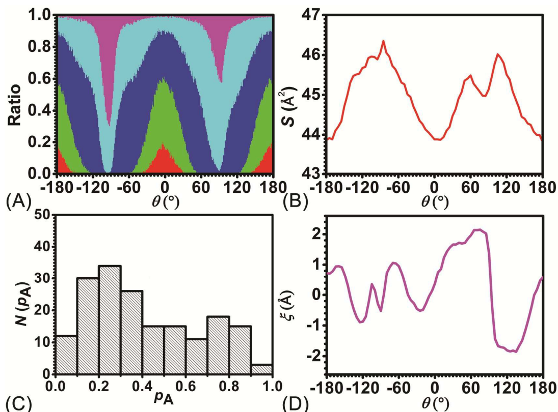
Figure 3. (A) The evolution of the percentage of conformations with 0-(magenta), 1-(cyan), 2-(blue), 3-(green), 4-(red) hydrogen bond(s) and (B) average area of the quadrilateral spanned by the center of the four benzyl units in the ring along the reaction coordinate, \theta . (C) Distribution of the committor, p_A ,
