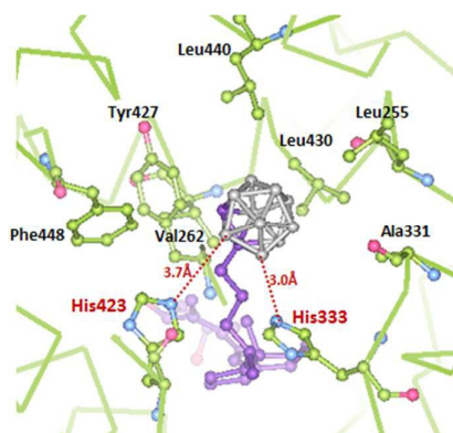
Figure 5 Details of the interactions mediated by the carborane moiety of ligand 1 with residues of the zVDR LBD at a 3.8 Å distance cutoff. Dihydrogen bonds between boron atoms and His333 and His423 are shown by red dashed lines. Distances are shown in Å.
