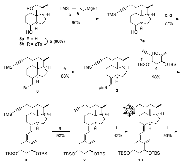
Scheme 2 Synthesis of target analog 1 . Reagents and conditions: a) p TsCl (1.5 equiv), py, 0 °C, 12 h; b) 6 (4 equiv), Et 2 O/THF (1:1); Li 2 CuCl 4 (0.01 equiv), THF, -78 °C → 23 °C, 12 h; c) Oxidation of 7a to the corresponding ketone 7b : PDC (3 equiv), CH 2 Cl 2 , 23 °C, 5 h; d) (Ph 3 PCH 2 Br)Br (8 equiv), toluene, ultrasound, 15 min; KOtBu in THF (7.9 equiv, 1 M), -15 °C → 0 °C, 2.5 h, then 7b in toluene, -15 °C → 23 °C, 3 h; e) Tol/THF (3:1), -78 °C, t BuLi (2 equiv), 1 h; B(O i Pr) 3 (1.5 equiv), 1.5 h; pinacol (1.3 equiv), -78 °C → 23 °C, 4 h; f) 4 (1 equiv), K 3 PO 4 (27 equiv, aqueous sol, 2 M), THF, PdCl 2 (PPh 3 ) 2 (0.05 equiv), 2 h; g) K 2 CO 3 , MeOH, 23 °C, 14 h; h) PhNMe 2 (6.5 equiv), toluene, decaborane (B 10 H 14 , 3 equiv), 110 °C, 1 h; i) HF (48%, 2.5 equiv), CH 2 Cl 2 /CH 3 CN (2:1), 23
