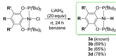
Scheme 4 Synthesis of the t Bu[POCOP]NiH Complexes.
