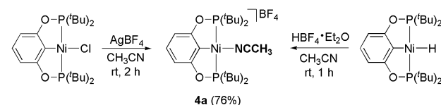
Scheme 5 Synthesis of the Nickel Pincer Acetonitrile Complexes.
