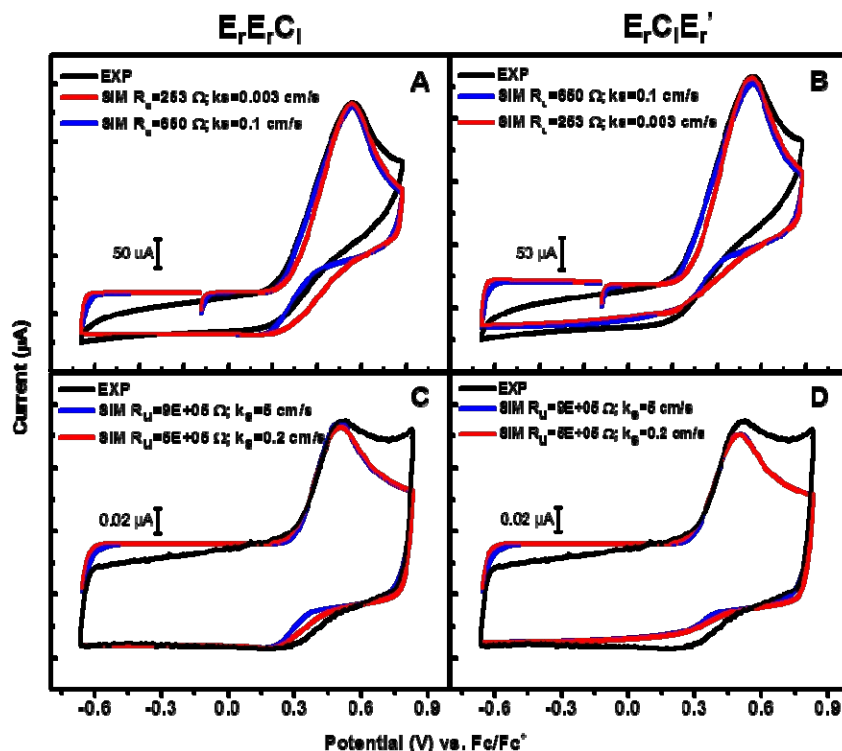
Fig. 6 Experiments and simulations of CVs of 3a at (A) and (B) 4 V/s with a 3 mm diameter working electrode; (C) and (D) 400 V/s with a 11 \mu\text{m} diameter working electrode. See supplementary information for details.
