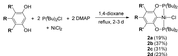
Scheme 4 Synthesis of the t Bu[POCOP]NiH Complexes.
