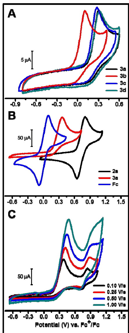
Fig. 2 (A) CV of 1 mM solutions of 3a-d in 1:4 by volume THF-MeCN (0.1 M TBABF 4 , TBA = Tetra- N -butyl ammonium) at 250 mV/s. (B) Comparison of CVs of 4 mM solutions of 2a , 3a and Ferrocene in 1:4 by volume THF-MeCN (0.1 M TBABF 4 ) measured at a scan rate of 250 mV/s. (C) CV of 3a beyond the first one-electron oxidation in THF (0.1 M TBABF 4 ) for different scan rates.
