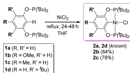
Scheme 3 Single-Pot Synthesis of the t Bu[POCOP]NiCl Complexes.
