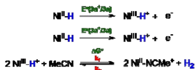
Scheme 6 Mechanisms for hydrogen production.
