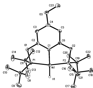
Fig. 1 X-ray Crystal Structure of 3b (50% probability level). Selected bond lengths ( \text{\AA} ) and angles (deg): Ni(1)–H(1) 1.47(2), Ni(1)–C(1) 1.8876(14), Ni(1)–P(1) 2.1155(6), Ni(1)–P(2) 2.1161(6), P(1)–Ni(1)–P(2) 165.288(17), C(1)–Ni(1)–H(1) 177.9(8), P(1)–Ni(1)–H(1) 95.7(8), P(2)–Ni(1)–H(1) 99.0(8).
