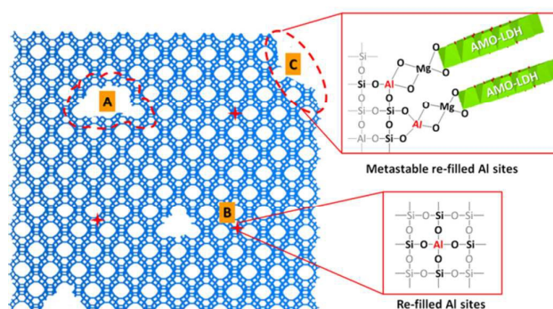
Figure 3. The proposed mechanism for the desilication of HY(5.1) and the formation of an AMO-Mg 2 Al-CO 3 -LDH coating on the zeolite surface.
