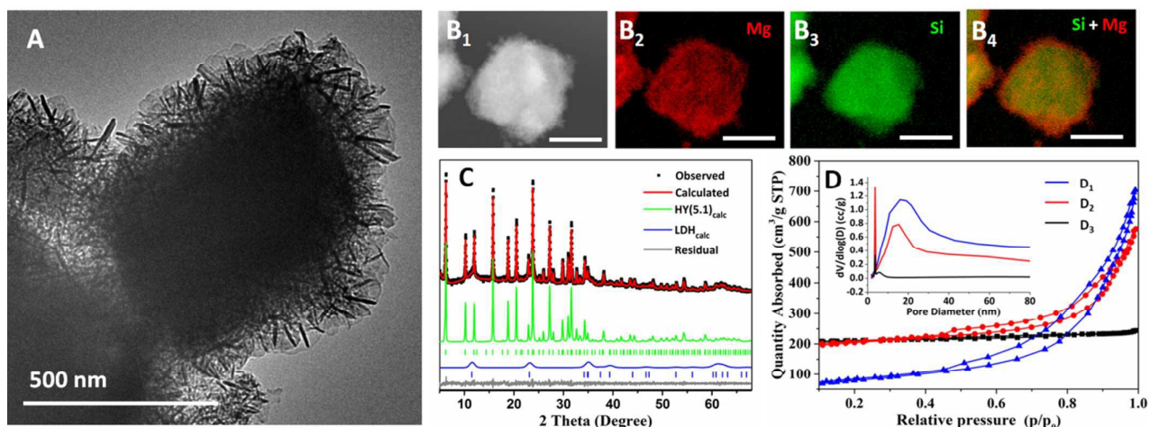
Figure 1. (A) TEM image of HY(5.1)@AMO-Mg 2 Al-CO 3 -LDH; (B 1 -B 4 ) STEM and EDX elemental mapping images of HY(5.1)@AMO-Mg 2 Al-CO 3 -LDH (the scale bars correspond to 500 nm); (C) XRD pattern and two-phase Pawley refinement of HY(5.1)@AMO-Mg 2 Al-CO 3 -LDH, showing the modelled HY(5.1) and LDH phases; (D) N 2 adsorption/desorption isotherms and pore size distribution (inset) of (D 1 ) AMO-Mg 2 Al-CO 3 -LDH, (D 2 ) HY(5.1)@AMO-Mg 2 Al-CO 3 -LDH and (D 3 )HY(5.1).
