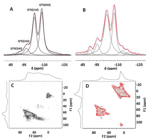
Figure 2 29 Si solid-state NMR of (A) HY(5.1) and (B) HY(5.1)@AMO-Mg 2 Al-CO 3 -LDH; 27 Al solid-state MQ MAS NMR of (C) HY(5.1) and (D) HY(5.1)@AMO-Mg 2 Al-CO 3 -LDH.
