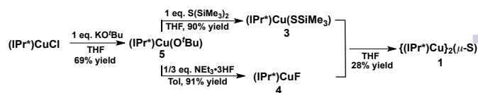
Scheme 2 Trimethylsilyl-deprotection route to 1 .
