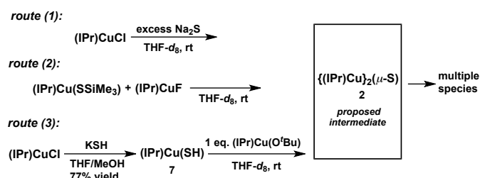
Scheme 4 Routes for the attempted synthesis of 2 .
