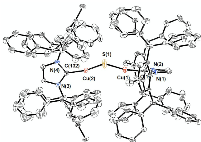
Fig. 1 X-ray crystal structure of 1 (50% probability ellipsoids). Hydrogen atoms are omitted for clarity. Selected bond lengths (Å) and bond angles ( ^\circ ): Cu(1)–C(1), 1.873(5); Cu(2)–C(132), 1.869(5); Cu(1)–S(1), 2.0787(17); Cu(2)–S(1), 2.0848(18); Cu(1)–Cu(2), 3.6085(9); C(1)–Cu(1)–S(1), 162.92(16); C(132)–Cu(2)–S(1), 158.81(16); Cu(1)–S(1)–Cu(2), 120.15(9). The dihedral angle between the IPr* imidazole rings is 89.9(3)^\circ .
