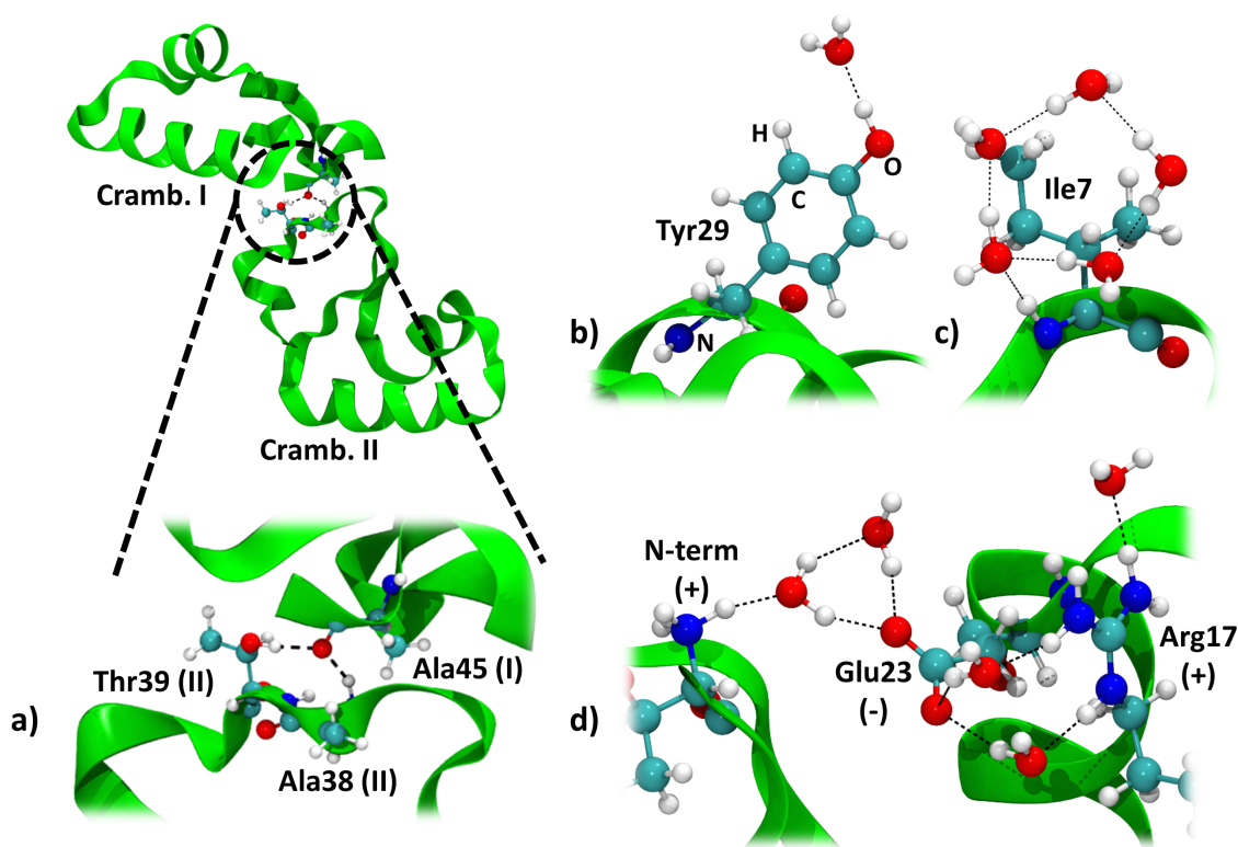
Figure 4. Main interactions in the crambin crystal. All views are from the 84W case (cf. Figure 2). a) Crambin-crambin interactions in the unit cell: overall view of the interaction and magnification of the involved residues. b) Water interacting with polar residues (Tyr29). c) Water arrangement around apolar residues (Ile7). d) Water
