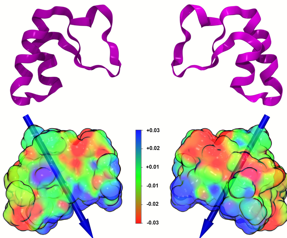
Figure 6. Electrostatic potential and dipole moment of crambin, as extracted from the 172W crystal structure. Left and right pictures are flipped by 180°. Top: ribbon view of crambin secondary structure. Bottom: electrostatic potential mapped on the B3LYP-D*/6-31G(d,p) electron density; an isosurface (isovalue = 0.0001 e) is shown. Blue, green and red colors correspond to positive, neutral, and negative values of the electrostatic potential (range values: MIN -0.03 au; MAX +0.03 au.). The computed dipole moment is represented as a
