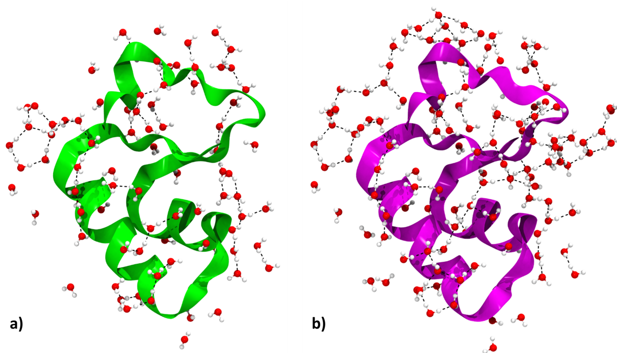
Figure 5. Crambin solvation shell, here defined as all the complete water molecules within 4 Å of any protein atom. a) Solvation shell of the 84W case (cf. Figure 2). b) Solvation shell of the 172W case (cf. Figure 2). Color code: red, oxygen; white, hydrogen; green, 84W protein backbone; magenta, 172W protein backbone; black, water-water H-bonds.
