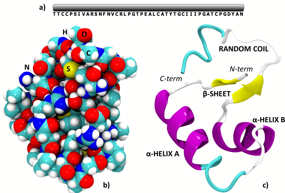
Figure 1. The structure of crambin. a) Primary structure; b) space-filled 3D model; c) secondary structure with indications of the main domains. PDB structure: 4FC1.
