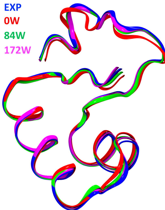
Figure 3. Comparison of crambin structures. Backbone as a ribbon representation. Color code: blue, experimental crystal structure (PDB: 4FC1); red, B3LYP-D*/6-31G(d,p) optimized crambin crystals with 0 H 2 O/cell; green, B3LYP-D*/6-31G(d,p) optimized crambin crystals with 84 H 2 O/cell, magenta, B3LYP-D*/6-31G(d,p) optimized crambin crystals with 172 H 2 O/cell.
