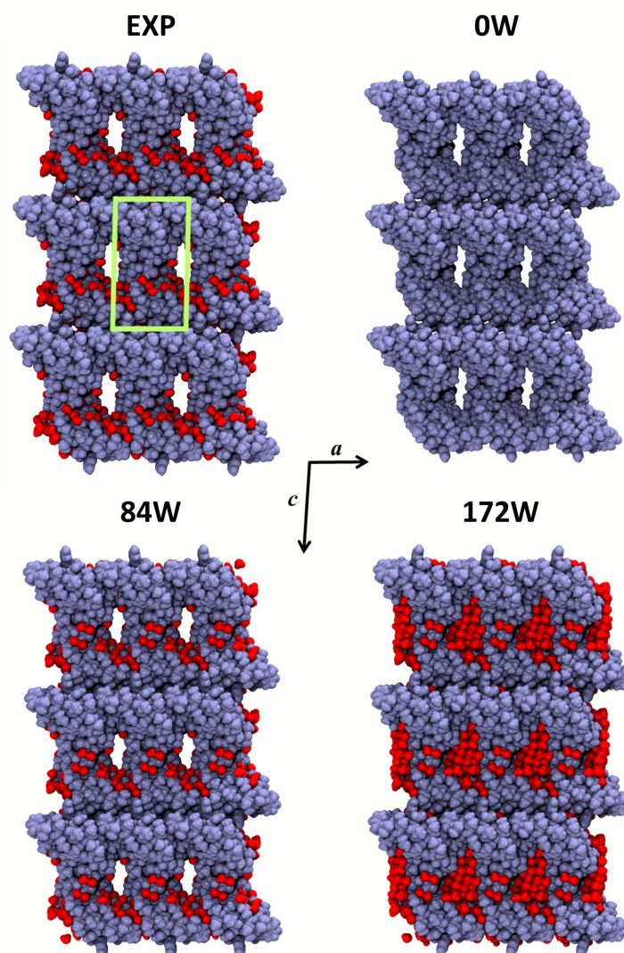
Figure 2. Crystal portion views of crambin. In all cases, a space-filled 3D view of a crystal box corresponding to 3 \times 3 \times 3 unit cells is reported (only complete molecules are shown), along the b axis. Color code: purple, protein atoms; red, water atoms; green, cell borders. EXP: experimental crystal structure (PDB: 4FC1); note that in this case only the 84 well-determined water molecules are shown, while the experimental crystal has a 30% water content (v/v). n W: B3LYP-D*/6-31G(d,p) optimized crambin crystals with n H 2 O/cell included in the simulation.
