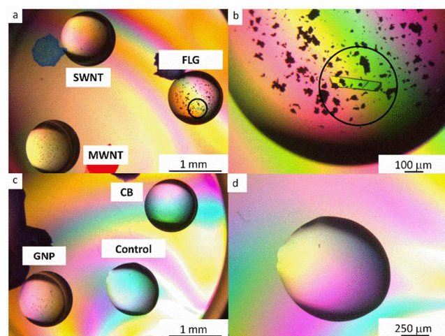
Fig. 2 Polarized optical microscopy of 30 mg ml -1 trypsin drops: a) and c) containing mPEG functionalized nanocarbons – FLG, SWNTs, MWNTs, GNPs and CB b) the circled single crystal formed within 24 h is surrounded by the FLG-mPEG flakes d) highlights the clear control after 72 h at this protein concentration and crystallization condition. The smaller, black features are agglomerates of functionalised CNMs. Other examples of protein crystals are available in Fig. S7.
