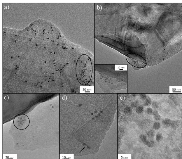
Fig. 3 TEM images of ferritin on FLG-mPEG: a) clusters of ferritin nanoparticles (circled) on stacked functionalized graphene layers; b-d) ferritin at edges and creases (inset in b and folds as indicated by arrows in d); e) higher resolution image of ferritin particles showing the lattice structure of Fe and clustering of ferritin.
