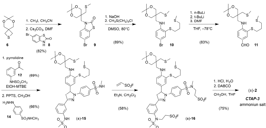
Scheme 1. Synthesis of fluorescent probe CTAP-3 (±)-2.
