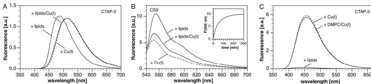
Figure 2 A) Fluorescence response of CTAP-2 ( \lambda_{\text{ex}} 380 nm) upon saturation with Cu(I) in the presence of DMPC/DMPG liposomes (4:1 mixture, 100 \mu\text{M} ) in pH 7.0 buffer at 25 ^{\circ}\text{C} (10 mM PIPES, 0.1 M \text{KClO}_4 , 100 nM MCL-1). B) Fluorescence response of Coppensor-3 (CS3, 2 \mu\text{M} ) under the same set of conditions ( \lambda_{\text{ex}} 530 nm). Inset: Time-dependent evolution of the fluorescence intensity at 550 nm prior to addition of Cu(I). C) Fluorescence response of CTAP-3 under the same set of condition used in (A) for CTAP-2 ( \lambda_{\text{ex}} 365 nm).
