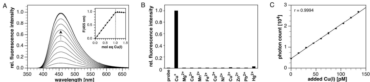
Figure 1. A) Titration of CTAP-3 (4 μM) in pH 6 buffer (10 mM MES, 100 nM MCL-1) with 0.4 μM aliquots of Cu(I) generated in situ by reduction of Cu(II)SO 4 with 100 μM sodium ascorbate ( \lambda_{\text{ex}} = 365 nm). B) Fluorescence response of CTAP-3 (4 μM) in pH 7 buffer (10 mM PIPES, 100 nM MCL-1) to divalent cations (concentration 20 μM, 10 mM Ca(II) and Mg(II)) and to Cu(I) generated by in situ reduction of 5 μM Cu(II) with 100 μM sodium ascorbate. The probe responded normally to Cu(I) in the presence of all competing ions (not shown). Excitation at 365 nm. C) Titration of CTAP-3 (2 nM) in ascorbate buffer (200 μM ascorbic acid, 170 μM KOH, 100 pM MCL-3) with 15 pM (0.95 part per trillion) aliquots of Cu(II)SO 4 reduced in situ to Cu(I). Excitation at 355 nm (10 nm monochromator bandpass) with 370/36 nm sharp cutoff bandpass filter. Emission collected at 455 nm (10 nm bandpass). Error bars represent the standard deviation over 6 successive 5-second measurements for each titration point.
