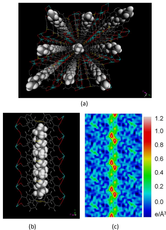
Fig. 3. View of n -hexane loaded structure. (a) Packing along the crystallographic b direction showing the location of n -hexane. Color scheme: calcium (cyan), sulfur (yellow), oxygen (red), carbon (grey), and hydrogen (white). (b) Packing of n -hexane molecules viewed along the crystallographic a direction; the hexane molecules can't be resolved as a single chemical entity. (c) The difference electron density map calculated before assigning the adsorbate, showing a continuous electron density ribbon along the channel.
