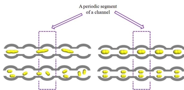
Fig. 1. Pictorial representation of commensurate and incommensurate adsorption within a tubular one-dimensional channel of a hypothetical MOF.
