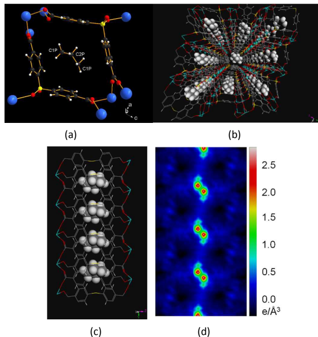
Fig. 2. View of propene loaded structure. (a) Local environment of propene inside the channel. (b) Projection view showing propene packing along the crystallographic b axis. Color scheme: calcium (cyan), sulfur (yellow), oxygen (red), carbon (grey), and hydrogen (white). (c) Packing of propene molecules viewed along the crystallographic a axis. The propene molecules are resolved as a single chemical entity. (d) The difference electron density map calculated before assigning the adsorbate; the island of positive electron density represents the propene molecule in the channel (the third C atom is out of plane).
