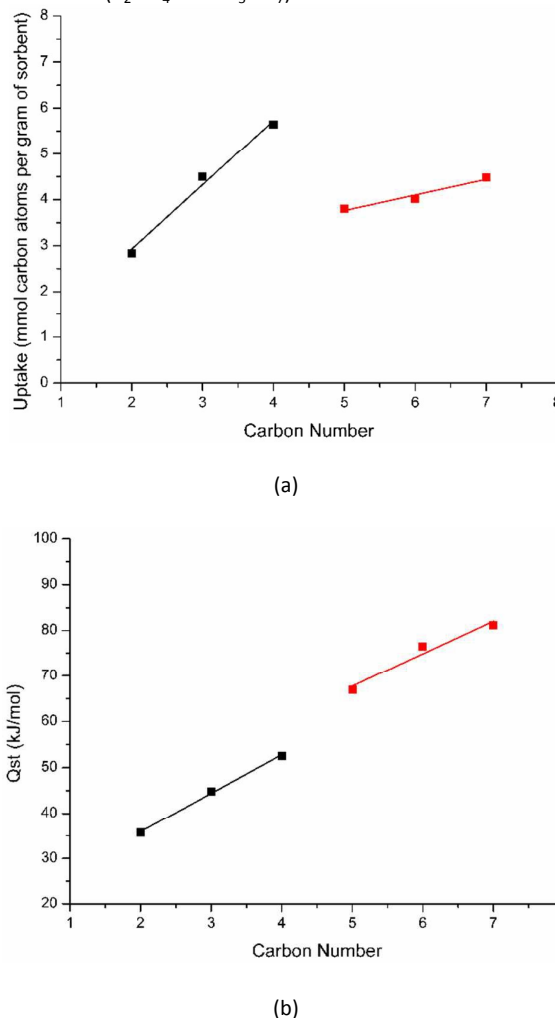
Fig. 4. (a) The uptake of hydrocarbons in 1' as a function of carbon numbers. (b) The Plot of Q_{st} values of hydrocarbons ( C_2 - C_7 ) in 1' as a function of carbon numbers. In the case of C_3^- , the value for C_3^- was used.
