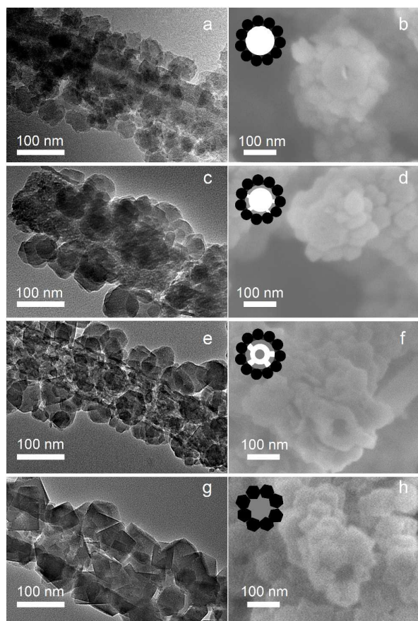
Fig. 4 Tracking the evolution of ZSM-5 nanotube using high magnification TEM and SEM: (a,b) 0 h. (c,d) 6 h. (e,f) 18 h. (g,h) 72 h.
