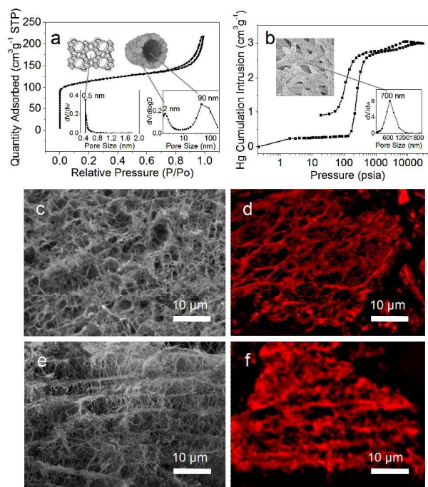
Fig. 3 Characterizing the scaffolding architecture of ZNTS ZSM-5: (a) N 2 sorption isotherm and micropore, mesopore and nanotube. (b) Hg intrusion porosimetry measurements and macropore profile. (c,e) Low magnification SEM and (d,f) LSCM images showing the anisotropic structure and the nanotubes connectivity, respectively.
