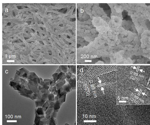
Fig. 2 Characterizing ZNTS ZSM-5: (a) Low magnification SEM showing nanotube scaffolding architecture. (b) High magnification SEM showing ZSM-5 nanotubes. (c) High magnification TEM showing nanotubes connectivity. (d) HRTEM showing the single crystal nature of ZSM-5. Inset: HRTEM showing the intergrowth between the adjacent nanocrystals of ZSM-5.
