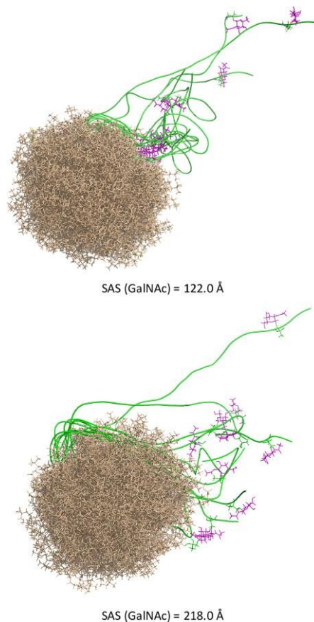
Fig 5. Ensembles obtained from 100 ns MD simulations on liposomes consisting of 65 dodecylphosphocholine lipids loaded with the threonine-containing lipoglycopeptide (upper panel) and derivative 1 (bottom panel). The peptide backbone is shown in
