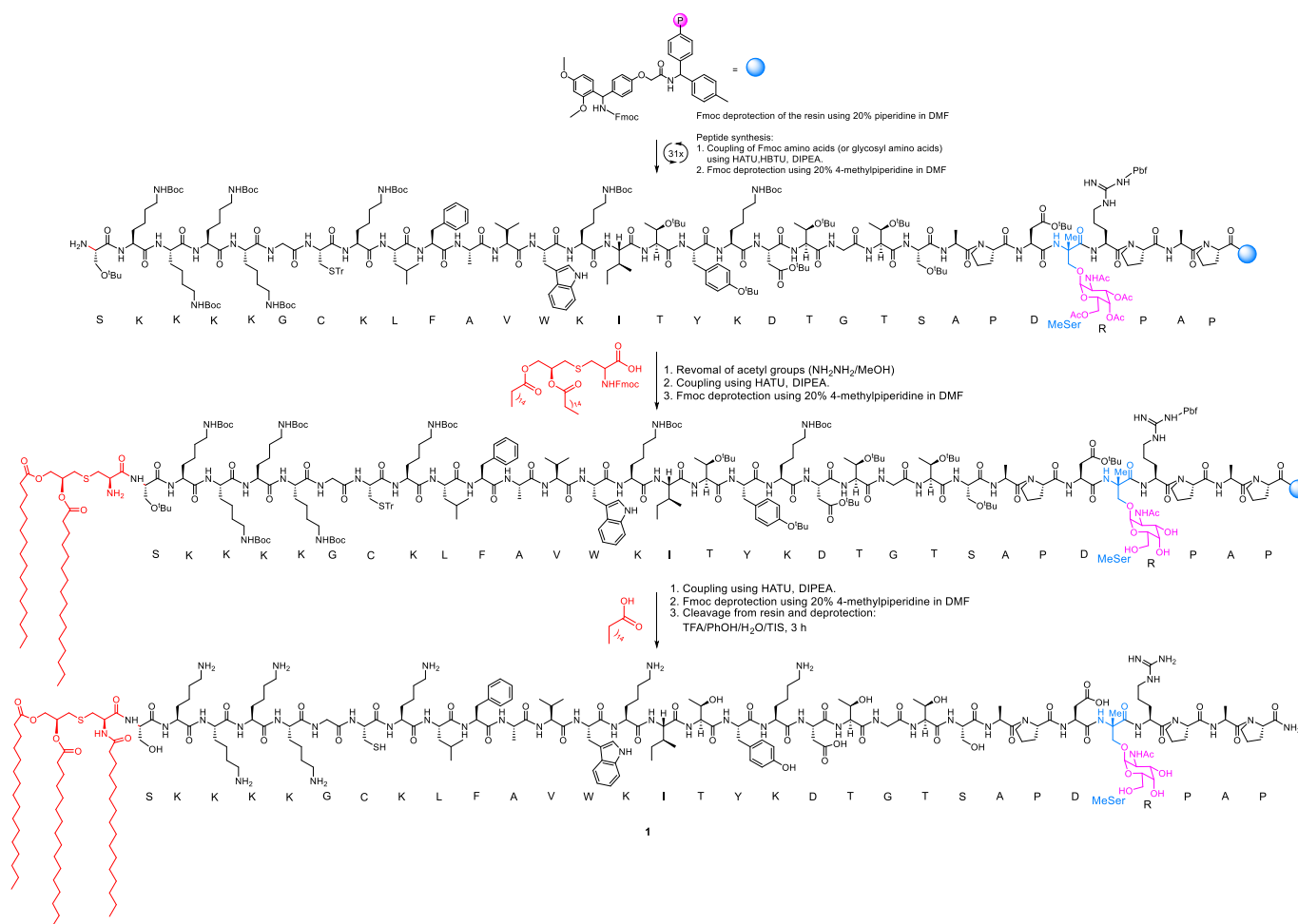
Scheme 2. Synthesis of vaccine 1 . The incorporation of building block 2 and the assembly of Fmoc-Pam 2 -Cys-OH were manually performed. HBTU= N,N,N',N' -Tetramethyl- O -(1H-benzotriazol-1-yl)uronium hexafluorophosphate. HATU= 1-[Bis(dimethylamino)methylene]-1 H -1,2,3-triazolo[4,5- b ]pyridinium 3-oxid hexafluorophosphate. DIPEA= N,N -diisopropylethylamine. TFA=trifluoroacetic acid. TIS=triisopropylsilane. DMF= N,N -dimethylformamide.
