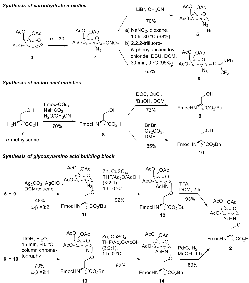
Scheme 1. Synthesis of building block 2.
