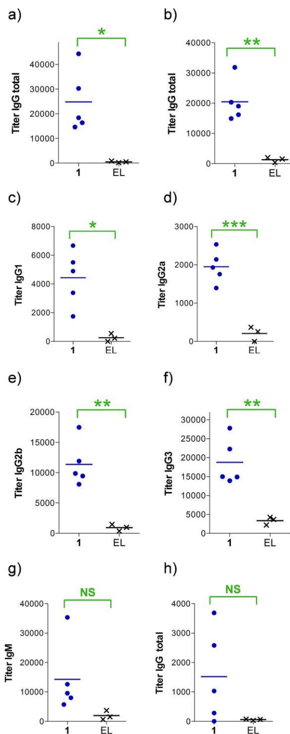
Fig 2. Anti-MUC1 and anti-T helper antibody titers after a) 3 or b-h) 4 immunizations with either empty liposomes (n=3) or vaccine 1 in liposomes (n=5) as indicated. ELISA plates were coated with a-g) BSA-MI-CTSAPDT( \alpha -D-GalNAc)RPAP conjugate or h) NeutrAvidin-biotin-T helper and titers were determined by linear regression analysis, plotting dilution vs. absorbance. Titers were defined as the highest dilution yielding an optical density of 0.1 or greater over that of normal control mouse sera. EL stands for empty liposomes. MI stands for maleimide. Each data point represents the titer for an individual mouse and the horizontal lines indicate the mean for the group of mice. Asterisks indicate statistically significant difference (*** P < 0.001, ** P < 0.01, * P < 0.05) and NS indicates no significant difference.
