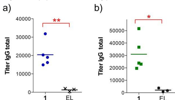
Fig 3. Anti-MUC1 (glycosylated and unglycosylated) antibody titers after 4 immunizations with either empty liposomes ( n=3 ) or vaccine 1 in liposomes ( n=5 ) as indicated. ELISA plates were coated with a) BSA-MI-CTSAPDT( \alpha -D-GalNAc)RPAP conjugate for anti-MUC1(Tn) titers or b) BSA-MI-CTSAPDTRPAP conjugate for anti-unglycosylated MUC1 titers. EL stands for empty liposomes. MI stands for maleimide. Each data point represents the titer for an individual mouse and the horizontal lines indicate the mean for the group of mice. Asterisks indicate statistically significant difference ( \star\star P<0.01 , \star P<0.05 ).
