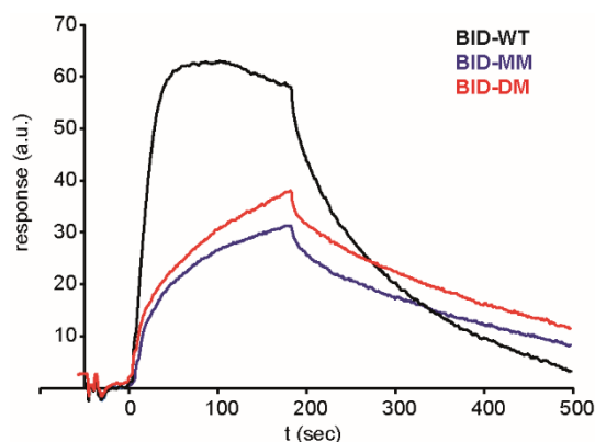
Figure 7. Surface plasmon resonance (SPR) sensorgram of BIM peptides at 100nM interacting with immobilised Bcl- \chi_L .
