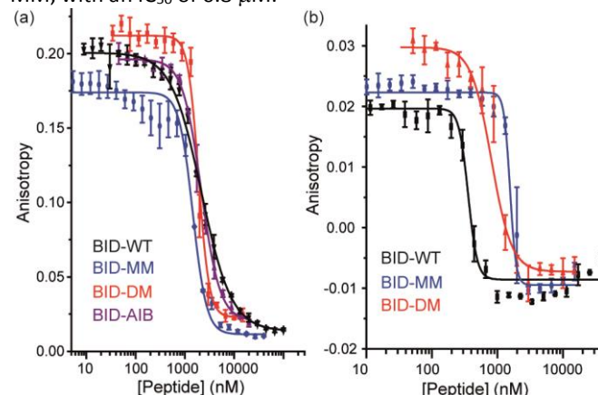
Figure 3. BID peptide/ protein titrations (a) fluorescence anisotropy competition assay for inhibition of Bcl-x L /BAK interaction, with Bcl-x L at 131nM and BODIPY-BAK at 43nM (b) fluorescence anisotropy competition assay for inhibition of Mcl-1/NOXA-B interaction, with Mcl-1 at 150nM and FITC-NOXA-B at 50nM (40 mM sodium phosphate, 200 mM sodium chloride, 0.02 mg ml -1 bovine serum albumin, pH 7.50).
