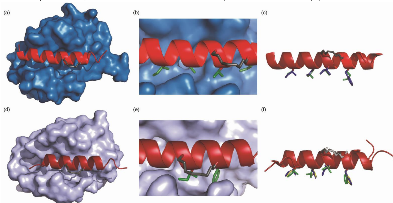
Figure 6. Crystal structures of constrained peptide/protein interactions (a) Mcl-1/BID-MM (PDB entry 5C3F) (b) enlargement of Mcl-1/BID-MM interface illustrating cis double bond and key side chains (c) overlay of BID-MM and Mcl-1/BIM-WT from PDB ID:2NL9 illustrating similarity of binding interface. Side chains from BID-MM are shown in green, with BIM-WT side chains in blue. (d) Bcl- \chi_L /BIM-MM (PDB entry 5C3G) (e) enlargement of Mcl-1/BID-MM interface illustrating cis double bond and key side chains (f) overlay of BIM-MM, BIM-WT (from PDB ID: 3FDL) and BIM-DM (from PDB ID: 2YQ6) illustrating similarity of binding interface Side chains from BIM-MM are shown in green, with BIM-WT side chains in blue and BIM-DM side chains in yellow.
