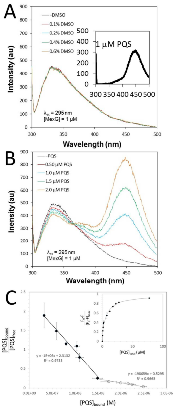
Figure 6. Fluorescence emission spectra of MexG and PQS. A. The fluorescence emission spectra of purified MexG ( 1 \mu\text{M} final concentration) was measured in the presence of the indicated amounts of added DMSO (DMSO was used as a solvent for PQS). The excitation wavelength was 295 nm. The highest final concentration of DMSO tested (0.6% v/v) was greater than the highest DMSO concentration achieved during the titration of PQS. Note that the addition of DMSO does not change the emission spectrum of MexG. Inset. Emission spectrum of 1 \mu\text{M} PQS excited at 295 nm. B. Emission spectrum of purified MexG in the presence of increasing concentrations of PQS. The excitation wavelength was 295 nm. Note how increasing PQS concentrations lead to an increase in emission at ca. 450 nm and a concomitant decrease (quenching) of emission at ca. 340 nm. C. Quantitation of PQS binding to MexG. Scatchard plot of the binding data derived from fluorescence quenching experiments. Note the biphasic binding behaviour of the MexG:PQS interaction, indicative of tight (filled symbols) and weaker (open symbols) binding interactions. The slope of each linear regression yields -1/K_d . Inset. The figure shows the fraction of protein fluorescence that was quenched at different total concentrations of added PQS.
