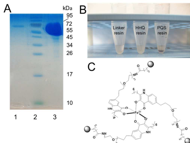
Figure 1. The PQS affinity probe retains affinity for PqsRLBD and Fe 3+ . A) Purified PqsR ligand binding domain (PqsRLBD) binds strongly to immobilized PQS but not to the control linker resin. Purified MBP-tagged PqsRLBD was incubated with aliquots of the control or PQS-derivatized resin, see ESI. The resin samples were extensively washed and the bound protein was eluted by boiling the washed beads in SDS sample buffer. The panel shows a Coomassie Brilliant Blue-stained SDS-PAGE gel of the protein eluting from control beads (lane 1) or PQS-derivatized beads (lane 3). Molecular mass markers are shown in lane 2. B) Aliquots (50 \mu L) of control beads, HHQ beads or PQS beads (as indicated) were mixed with 1 mM FeCl 3 . The PQS beads immediately turned deep red due to the formation of the PQS-iron complex. C) Proposed structure of the PQS-Fe complex on probe resulting in dark red colouration.
