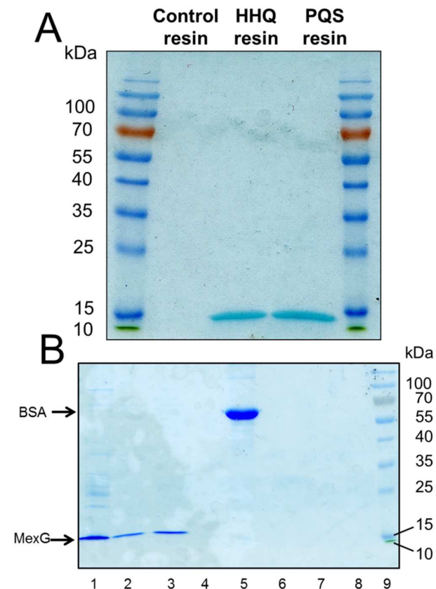
Figure 4. Purified MexG binds to immobilized PQS and immobilized HHQ in vitro. A. Purified MexG was incubated with either linker resin, HHQ or PQS affinity probes (as indicated) for 1 h. After extensive washing of the resins, the bound protein was eluted in SDS sample buffer and resolved by SDS-PAGE. The resulting Coomassie Brilliant Blue-stained gel is shown. B. The experiment in (A) was repeated using BSA in place of MexG. Lane 1; An aliquot of the MexG sample that was loaded onto the resin, lane 2; MexG bound to PQS resin, Lane 3; MexG bound to HHQ resin, Lane 4; MexG bound to control resin, Lane 5; BSA alone, Lane 6; BSA bound to PQS resin, Lane 7; BSA bound to HHQ resin, Lane 8; BSA bound to control resin, Lane 9; molecular mass markers.
