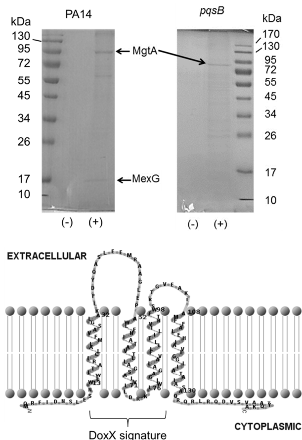
Figure 2. The PQS affinity probe captures MgtA and MexG from the detergent-solubilized cell membrane fraction. Detergent-solubilized cell membranes from stationary phase cultures of wild-type PA14 or an isogenic pqsB mutant, as indicated, were mixed with aliquots of either control resin (-) or PQS resin (+). Following extensive washing of the resins, bound proteins were eluted by boiling the resin samples in SDS sample buffer. The eluted proteins were resolved by SDS-PAGE and an image of the Coomassie Brilliant Blue-stained gel is shown. Following staining of the gel, a selection of bands were excised and identified by MALDI-MS. The MgtA and MexG-containing bands are indicated. Predicted membrane topology of MexG. The DoxX domain (residues 15-95, encompassing most of helices 1-3) signature is indicated. The MexG amino acid sequence was analysed by TMHMM and the output was depicted using TMRPRES2D.
