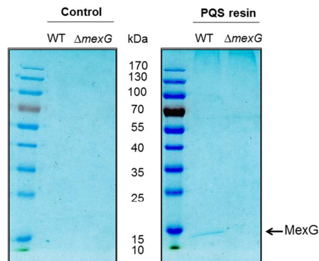
Figure 3. Deletion of the DoxX motif abolishes MexG binding to PQS. Detergent-solubilized membranes from either wild-type PAO1 or from an in-frame mexG deletion mutant (as indicated) were mixed with control resin or PQS-derivatized resin and incubated to allow binding. The resins were washed extensively and the bound proteins were eluted by boiling in SDS sample buffer. The figure shows a Coomassie Brilliant Blue-stained gel of the proteins bound to control resin (left panel) and PQS resin (right panel). Note that essentially the only protein detectable in this experiment was MexG from the wild-type extract bound to the PQS resin. Control = Linker only resin.
