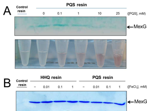
Figure 4. Purified MexG binds to immobilized PQS and immobilized HHQ in vitro. A. Purified MexG was incubated with either linker resin, HHQ or PQS affinity probes (as indicated) for 1 h. After extensive washing of the resins, the bound protein was eluted in SDS sample buffer and resolved by SDS-PAGE. The resulting Coomassie Brilliant Blue-stained gel is shown. B. The experiment in (A) was repeated using BSA in place of MexG. Lane 1; An aliquot of the MexG sample that was loaded onto the resin, lane 2; MexG bound to PQS resin, Lane 3; MexG bound to HHQ resin, Lane 4; MexG bound to control resin, Lane 5; BSA alone, Lane 6; BSA bound to PQS resin, Lane 7; BSA bound to HHQ resin, Lane 8; BSA bound to control resin, Lane 9; molecular mass markers.
