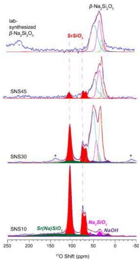
Fig. 3. ^{17}\text{O} MAS NMR spectra of SNS10, SNS30, SNS45, and lab-synthesized \beta\text{-Na}_2\text{Si}_2\text{O}_5 . All the samples are ^{17}\text{O} -isotope enriched, except the synthesized \beta\text{-Na}_2\text{Si}_2\text{O}_5 . Relevant resonance assignments, including \text{SrSiO}_3 (red), \text{SrSiO}_3 with Na doped within the structure ( \text{Sr}(\text{Na})\text{SiO}_3 , green), \text{Na}_2\text{SiO}_3 (magenta), NaOH (purple), and \beta\text{-Na}_2\text{Si}_2\text{O}_5 (cyan and blue lines) are marked on the spectra. Spectral simulations (red lines) are displayed together with the experimental spectra (blue lines). All the parameters used for the simulations are listed in Table S3. * marks the spinning sidebands. + denotes the one of the spinning sidebands from the ^{17}\text{O} NMR resonance of \text{ZrO}_2 rotor at 370 ppm.
