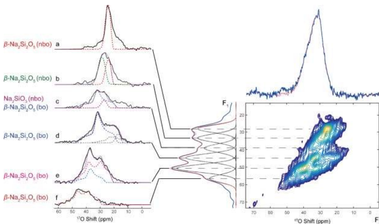
Fig. 4. ^{17}\text{O} multiple-quantum magic-angle spinning (MQMAS) NMR of ^{17}\text{O} isotope-enriched SNS45. The 1D quadrupolar patterns, labelled with a, b, c, d, e, and f, are cross sections from the 2D spectrum taken at the positions marked with dashed lines. Simulated patterns are overlapped with the cross sections. The purple dashed lines represent the sum of all simulated quadrupolar patterns for each spectrum in a-f. The spectra on the top (red) and left (blue) of the 2D MQMAS spectrum are projections of the respective dimensions. The projection on the left (blue) is a sum of the isotropic spectra of various O sites and the simulated spectrum of each O site is also displayed (dotted lines under the projection spectrum). The projection (red) on the top of the 2D spectrum is overlapped with the regular MAS spectrum obtained at the same spinning speed as the MQMAS, i.e., 10 kHz MAS.
