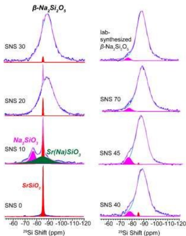
Fig. 1. 29 Si MAS NMR spectra of Na-doped SrSiO 3 (with apparent compositions of Na x Sr 1-x SiO 3-0.5x ) with different Na contents (x = 0, 0.1, 0.2, 0.3, 0.4, 0.45, and 0.70, denoted as SNS0, SNS10, SNS20, SNS30, SNS40, SNS45, and SNS70, respectively) and lab-synthesized β-Na 2 Si 2 O 5 . Relevant resonance assignments, including SrSiO 3 (red), SrSiO 3 with Na doped within the structure (Sr(Na)SiO 3 , green), Na 2 SiO 3 (magenta), and β-Na 2 Si 2 O 5 (blue) are marked on the spectra. Spectral simulations are displayed together with the experimental spectra. All the NMR parameters used for the simulations are listed in Table S1.
