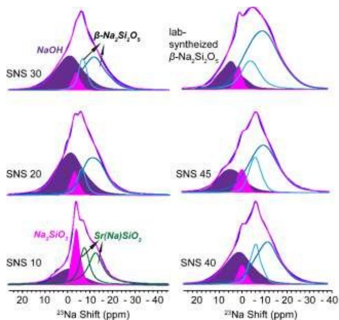
Fig. 2. ^{23}\text{Na} MAS NMR spectra of SNS10, SNS20, SNS30, SNS40, SNS45, and lab-synthesized \beta\text{-Na}_2\text{Si}_2\text{O}_5 . Relevant resonance assignments, including \text{SrSiO}_3 with Na doped within the structure ( \text{Sr}(\text{Na})\text{SiO}_3 , green), \text{Na}_2\text{SiO}_3 (magenta), NaOH (purple), and \beta\text{-Na}_2\text{Si}_2\text{O}_5 (cyan and blue) are marked on the spectra. Spectral simulations are displayed together with the experimental spectra. All the parameters used for the simulations are listed in Table S2.
