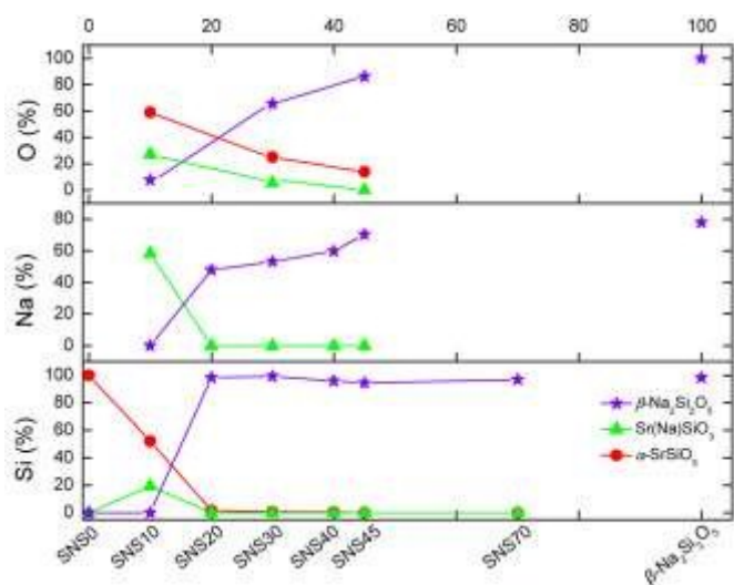
Fig. 5. Quantification of Si, Na, and O in various chemical phases in SNS samples based on the area integral of the ^{29}\text{Si} , ^{23}\text{Na} , and ^{17}\text{O} NMR spectra in Figures 1, 2, and 3.
