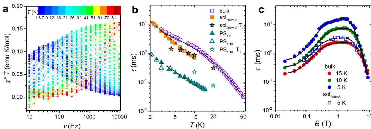
Figure 2. a) Frequency dependence of the imaginary component of the AC susceptibility of 1bulk in B_{dc}=0.2 T multiplied by temperature to be readable in the whole 2-80 K temperature range. b) Temperature dependence of the relaxation time of the magnetic susceptibility measured in B_{dc}=0.2 T for the pure and the diluted samples of 1: two dispersions in polystyrene with 1:5 and 1:10 mass ratio and a 200 mM \text{CH}_2\text{Cl}_2 :toluene frozen solution (see legend). The black solid line corresponds to the best fit of the bulk data using eq. 1, while the broken lines correspond to simulation with T^n law. T_1 for the diluted sample, extracted from pulsed EPR spectra, are shown for comparison. c) Field dependence of the relaxation time of the magnetic susceptibility of the bulk and the 200mM frozen solution sample (see legend). The solid lines represent the best fit obtained with eq. 3. Best fit parameters are reported in Table 1.
