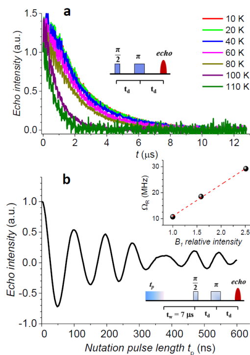
Figure 4. a) Pulsed EPR Hahn echo decay traces for 1\text{sol}_{1\text{mM}} at different temperatures recorded at 343 mT. In the inset the employed pulse sequence. b) Rabi oscillations for 1\text{sol}_{1\text{mM}} recorded at 4.3 K at 10 dB microwave attenuation. The change in oscillations observed at t_p > 400 ns is due to the interaction between the electron spin and surrounding protons. 48 In the inset the Rabi frequency ( \Omega_R ) vs oscillating field intensity superimposed to the linear best-fit.
