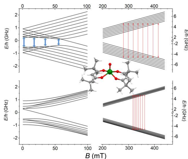
Figure 1. Zeeman splitting of the S=1/2 , I=7/2 manifold calculated with the field applied along the largest hyperfine coupling component (upper) and along the smallest (lower) (parameter in the text). Red lines correspond to the observed X-band ( \nu=9.62 GHz) EPR transitions while in pale blue are drawn the potential low frequency transitions at the avoided level crossings. In the inset the molecular structure of \text{VO}(\text{dpm})_2 .
