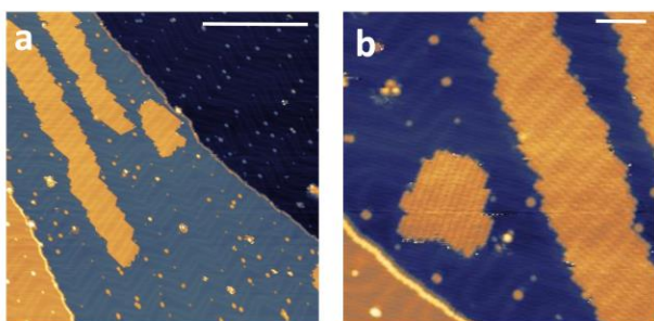
Figure 5. STM images of a sub-monolayer deposition of \text{VO}(\text{dpm})_2 measured at 30 K. Bias voltage = -2V (empty states), tunnelling current = 5 pA. The scanned regions are 150×150 nm in (a) and 60×60 nm in (b) and the bars correspond to 50 nm and 10 nm, respectively.
