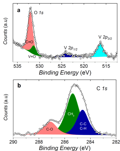
Figure 6. XPS spectra of a monolayer coverage of 1 on Au(111). The O 1s and V 2p regions are shown in (a) while the C 1s region in (b). Filled area and lines represent the best fit components and resulting spectra, respectively.
