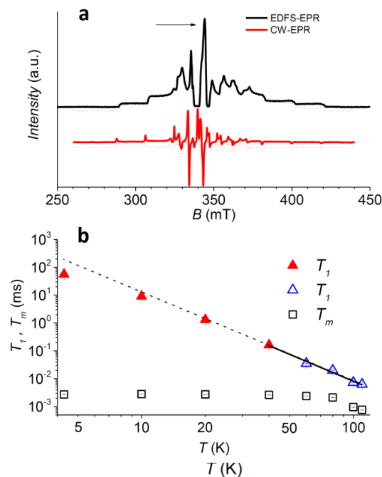
Figure 3. a) Echo detected (black trace) and CW (red trace) experimental EPR spectra of 1sol 1mM , measured at 5 K, and best simulations (dotted traces). The arrow marks the field position of T_1 and T_m determination. b) Temperature dependence of T_1 and T_m for 1sol 1mM sample. Full symbols refer to experiments of echo saturation by fast repetition, empty ones to inversion recovery experiments (See ESI for details). The solid line corresponds to the best-fit of the high temperature data with T_1 \propto T^n .
