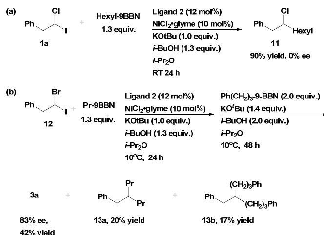
Scheme 3. (a) Generation of the racemic intermediate 11 (b) Enantioselective alkyl-alkyl Suzuki cross-coupling of geminal bromo-iodoalkane 12 .
