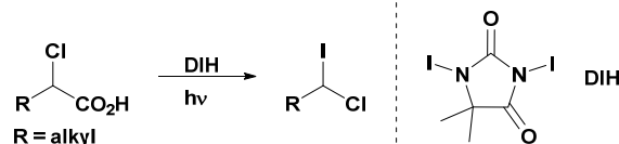
Scheme 2. Synthesis of geminal chloro(iodo)alkanes via iododecarboxylation of \alpha -chloroalkanoic acids.
