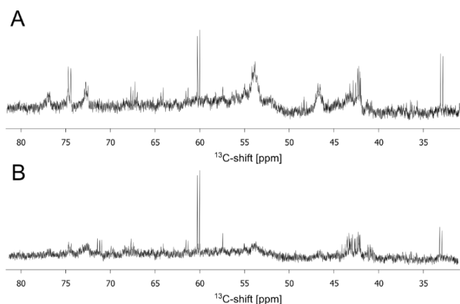
Fig. 5. Extract of the ^{13}\text{C} spectra of unlabelled DERA after incubation with ^{13}\text{C} -labeled acetaldehyde. (A) 1D spectrum recorded after removal of free reaction products. (B) The same sample after a heating step of 4 h at 50 °C. A negative control of DERA without substrate incubation (not shown) was used to exclude misinterpretation of signals due to the natural abundance of ^{13}\text{C} within the protein.
