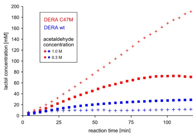
Fig. 10. Time dependent lactol 3 (compound 3 in Fig. 4) formation by wildtype DERA vs its C47M mutant. Product concentrations were determined via integration of ^1\text{H} -signals in the NMR spectra. More detailed analyses regarding substrate conversion and formation of the single aldol product are given as Supplementary Information, Fig S11.
