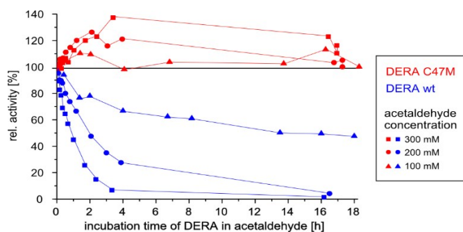
Fig. 9. Time-dependent activity of wildtype vs. C47M DERA during incubation at different acetaldehyde concentrations.
