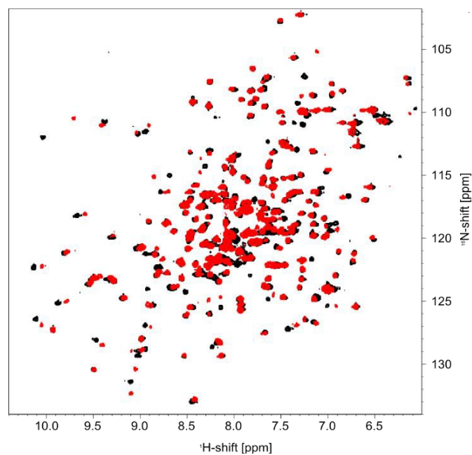
Fig. 2. [ 1 H, 15 N]-TROSY spectrum of [ U - 15 N] monomeric DERA recorded before (black) and after (red) treatment with acetaldehyde
