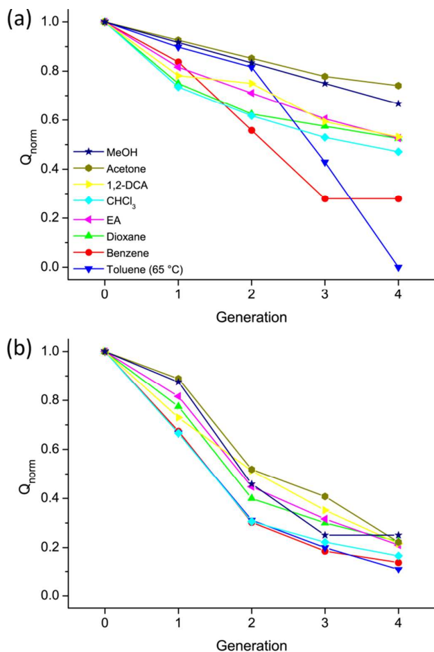
Fig. 5 Comparison of degree of swelling Q_{norm} versus g for hs-PGg (a) and ls-PGg (b) in various solvents at room temperature (except for toluene).
