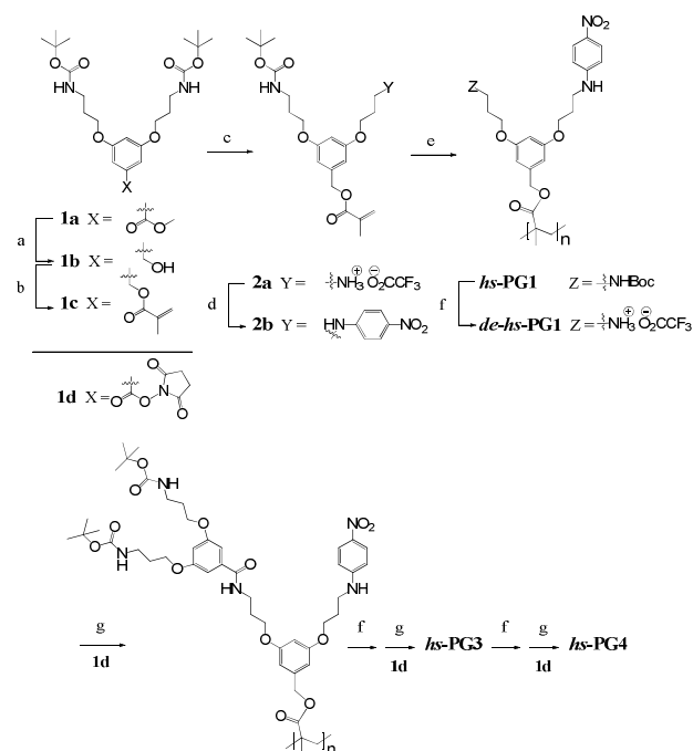
Scheme 1 Synthesis of homopolymer series hs-PG1 to hs-PG4 . Reagents, conditions and yields: a) LAH, THF, 2 h, 88%. b) methacryloyl chloride, Et 3 N, DMAP, DCM, 2 h, 76%. c) TFA, DCM, 4 d, 59%. d) p -Fluoronitrobenzene, Et 3 N, DMF, 65 °C, 15 h, 70%. e) AIBN, DMF, 65 °C, 15 h, 66%. f) TFA, 15 h, ~100%. g) 1d , Et 3 N, DMAP, DMF, 6-20 d, 65-85 %.
