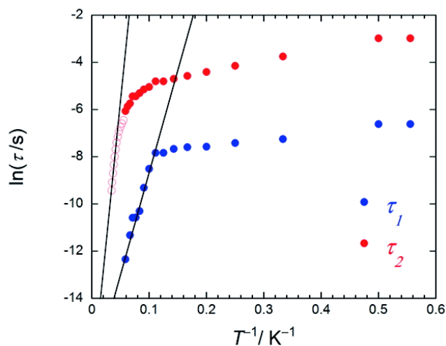
Fig. 6 An Arrhenius plot of 2 (SAP-SAP*), where the magnetic relaxation time \tau (blue and red circles) were obtained from \chi_M'' versus \nu plots (Fig. S26b) at T between 1.8 and 20 K in an H_{dc} of 1000 Oe and the red open circles were obtained from peak top T of \chi_M''T versus T plots (Fig. 4c) at T between 22 and 27 K in an H_{dc} of 1000 Oe. \tau was obtained from the least-squares fitting using a generalized Debye model (eq. S4–S6) and an extended Debye model (eq. S8–S10).
