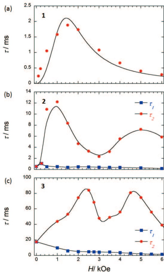
Fig. 8 \tau versus H for (a) 1 (SP-SP), (b) 2 (SAP-SAP*), and (c) 3 (SAP-SAP) 6 at 5 K. \tau was obtained from the least-squares fitting using an extended Debye model (eq. S8-S10 and Figs. S20 and S28). The order of the maximum values of \tau (red circle) are different from each other. See main text. The solid lines are guides for eyes.
