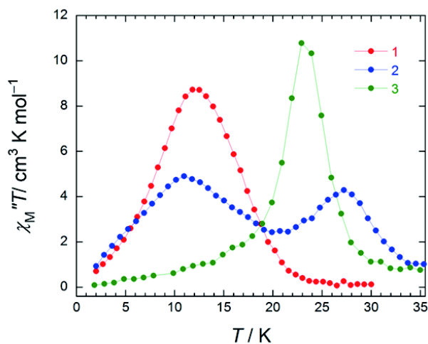
Fig. 5 Temperature ( T ) dependence of the ac magnetic susceptibilities ( \chi_M'' : out-of-phase) of 1–3 ( \chi_M''T versus T plot). The measurements were performed in a 3 Oe ac magnetic field at the indicated frequencies (996 Hz) in an H_{dc} of 1000 Oe for 1 (SA-SP), 1500 Oe for 2 (SAP-SAP*), and zero for 3 (SAP-SAP), respectively. In order to suppress QTM, we applied an H_{dc} for 1 and 2 (see main text). The solid lines are guides for eyes.
