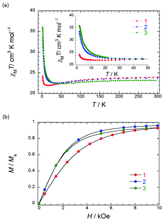
Fig. 2 (a) Temperature ( T ) dependence of \chi_M T measured on powder samples of 1 (SP-SP), 2 (SAP-SAP*) and 3 (SAP-SAP) at 500 Oe. (b) Normalised magnetization versus field ( M/M_s versus H ) performed on powder samples of 1–3 . The solid lines are guides for eyes.
