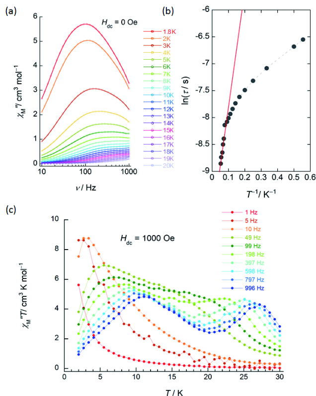
Fig. 4 Frequency ( \nu ) and temperature ( T ) dependence of the ac magnetic susceptibility ( \chi_M'' : out-of-phase) of 2 (SAP-SAP*). The measurements were performed in a 3 Oe ac magnetic field at the indicated \nu . (a) \nu dependence of \chi_M'' measured between 1.8 and 20 K in an H_{dc} of zero. The solid lines are guides for eyes. (b) Arrhenius plots for 2 in an H_{dc} of zero. Solid lines were fitted by using the Arrhenius equation (see main text). (c) \nu dependence of \chi_M'' T versus T at H_{dc} of 1000 Oe. The solid lines are guides for eyes.
