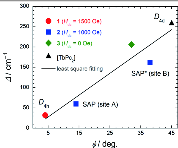
Fig. 7 The relationship between the twist angle ( \varphi ) and the energy barrier for the reversal of the magnetization ( \Delta ). The experimental data for [TbPc 2 ] - complex with D_{4d} geometry from ref. 4c and 3 from ref. 7e. In order to suppress QTM, we applied an H_{dc} for 1 and 2 (see main text). The solid line is a guide for eyes.
