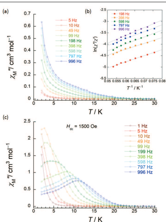
Fig. 3 Frequency ( \nu ) and temperature ( T ) dependence of the ac magnetic susceptibilities ( \chi_M'' : out-of-phase) of 1 (SP-SP). The measurements were performed in a 3 Oe ac magnetic field at the indicated frequencies in an H_{dc} of (a) zero. The solid lines are guides for eyes. (b) \chi_M''/\chi_M' versus T^{-1} (13–18 K) plot at the given \nu (198–996 Hz) of the ac susceptibility data by using the Kramers-Kronig equation (eq. S1–S3). The solid lines were fitted as described in Table S2. (c) \nu dependence of \chi_M'' versus T in an H_{dc} of 1500 Oe. The solid lines are guides for eyes.
