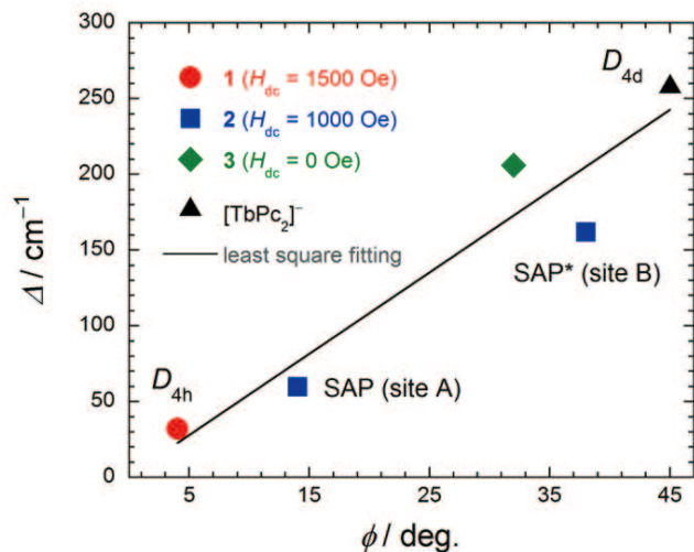
Fig. 7 The relationship between the twist angle ( \phi ) and the energy barrier for the reversal of the magnetization ( \Delta ). The experimental data for [\text{TbPc}_2]^- complex with D_{4d} geometry from ref. 4c and 3 from ref. 7e. In order to suppress QTM, we applied an H_{\text{dc}} for 1 and 2 (see main text). The solid line is a guide for eyes.
