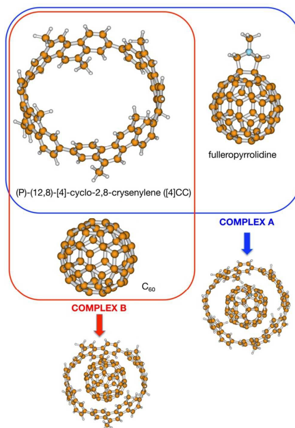
Figure 1. Species considered in this work.
