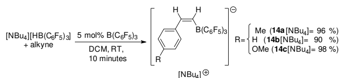
Scheme 7: Alkyne trans -hydroboration with \text{B}(\text{C}_6\text{F}_5)_3 / [\text{HB}(\text{C}_6\text{F}_5)_3]^-
