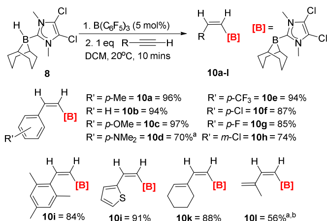
Scheme 3. Reaction scope and isolated yields (unless otherwise stated) for the trans -hydroboration of terminal alkynes. a = yield by NMR spectroscopy versus mesitylene as internal standard. b = 10 mol % \text{B}(\text{C}_6\text{F}_5)_3 .
