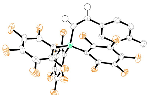
Figure 3: ORTEP depiction of [ 14a ] (thermal ellipsoids at 50%)
