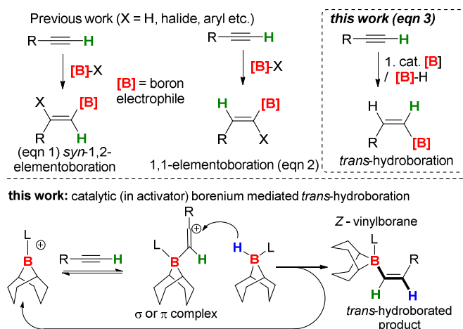
Figure 1: Previous work on alkyne elemento-boration (eqn. 1 and 2), and the work described herein (eqn. 3). Bottom, intermolecular hydride transfer for trans -hydroboration (intermediate shown as a vinyl cation a \pi complex between borenium and alkyne is also feasible).
