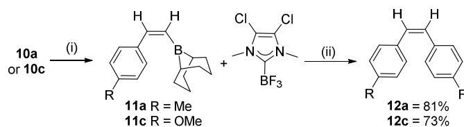
Scheme 4. Suzuki Miyaura cross coupling of 10x . (i) 1 equiv. \text{BF}_3(\text{OEt}_2) , toluene, 60°C, 1 h. (ii) Dried in-vacuo , then \text{Pd}(\text{P}^t\text{Bu}_3)_2 (10 mol%), 4-iodo-fluorobenzene (1.1. eq.), THF, \text{KO}^t\text{Bu} (2.5 eq.) 20°C, 18 h.
