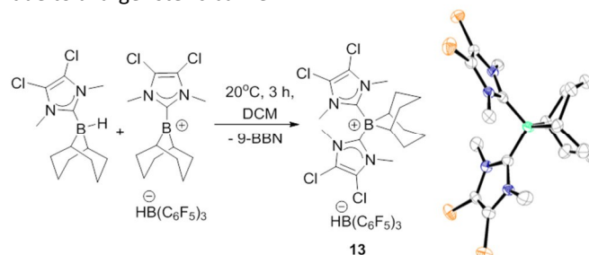
Figure 2. Formation of 13 and structure of 13 (thermal ellipsoids at 50% probability). Hydrogens and [HB(C_6F_5)_3]^- omitted for clarity.
