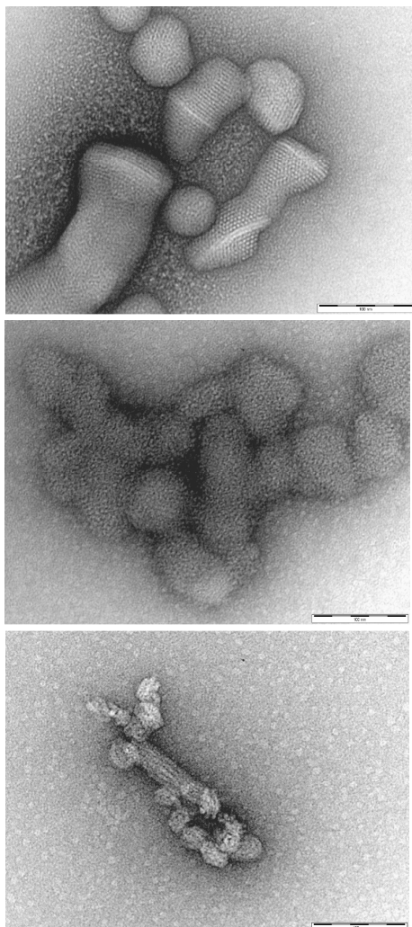
Figure 4. TEM images of self-assembled micellar nanostructures binding to heparin to yield a hierarchically organised self-assembled nanoscale aggregate and supporting the view that self-assembled micelles remain stable under polyanion binding conditions: (top) C_{16} -DAPMA, (middle) C_{16} -SPD, (bottom) C_{16} -SPM. All scale bars are 100 nm.
