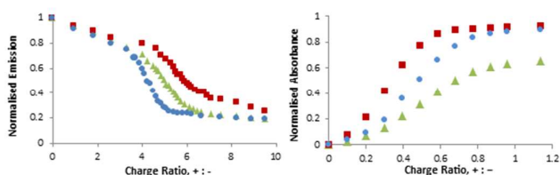
Figure 3. Titration curves for EthBr (left, DNA Binding) and MaIB (right, heparin binding) displacement. For DNA binding: [DNA] = 4 μM (per base), [EthBr] = 5.07 μM, buffer: 2 mM HEPES, 0.05 mM EDTA, 150 mM NaCl. For heparin binding: [heparin] = 27 μM (per disaccharide unit), [MaIB] = 25 μM, buffer: Tris HCl 10 mM, 150 mM NaCl. Blue = C 16 -SPM, Red = C 16 -SPD, Green = C 16 -DAPMA.
