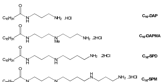
Figure 1. Compounds investigated in this paper.
