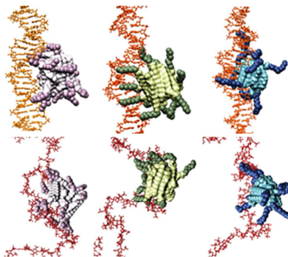
Figure 5. Equilibrated atomistic molecular dynamics (MD) simulation snapshots of SAMul micelles binding DNA (upper panel, orange) and heparin (lower panel, firebrick). In both panels, from left to right: C_{16} -DAPMA (light grey ( C_{16} ) and plum (DAPMA)), C_{16} -SPD (lime green ( C_{16} ) and forest green (SPD)), and C_{16} -SPM (steel blue ( C_{16} ) and navy blue (SPM)). Hydrogen atoms, water molecules, ions and counterions are not shown for clarity.
