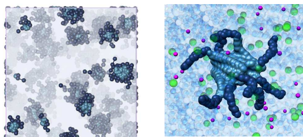
Figure 2. Mesoscopic (left) and atomistic (right) simulations of C 16 -SPM self-assembling into micelles. The C 16 hydrophobic portion is shown as steel blue spheres whereas the SPM residues are portrayed as navy blue spheres. In the left panel, water, ions and counterions are shown as light grey field; in the right panel, water molecules are depicted as transparent light blue spheres, some Na + and Cl - ions are shown as purple and green spheres, respectively.
