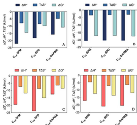
Figure 6. Charge-normalized per-residue effective free energy of binding ( \Delta G^* ), and enthalpic ( \Delta H^* ) and entropic ( T\Delta S^* ) components for: (A) each SAMul micelle ligand-type complexed with DNA; (B) DNA-bases complexed with each of the SAMul micelles; (C) each SAMul micelle ligand-type complexed with heparin; (D) heparin sugars complexed with each of the SAMul micelles.
