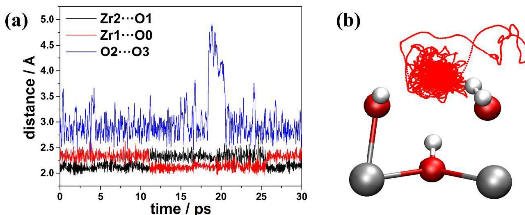
Figure 3: (a) Changes of distances (in Å) and (b) trajectory of the O3 atom (represented by red dotted line) during the AIMD simulation at 300 K.
