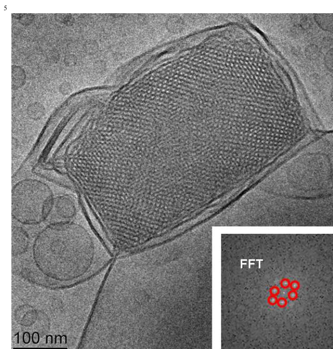
Figure 3. Cryo-TEM image of a cubosome nanoparticle with traditional (non-swollen) aqueous channels yielding well defined diffraction peaks in the Fast Fourier Transform (FFT) pattern (inset). The red colour in the inset highlights the FFT image analysis. This nanocarrier does not include a cationic lipid ( i.e. the particle was obtained at 0 mol.% DOMA).
