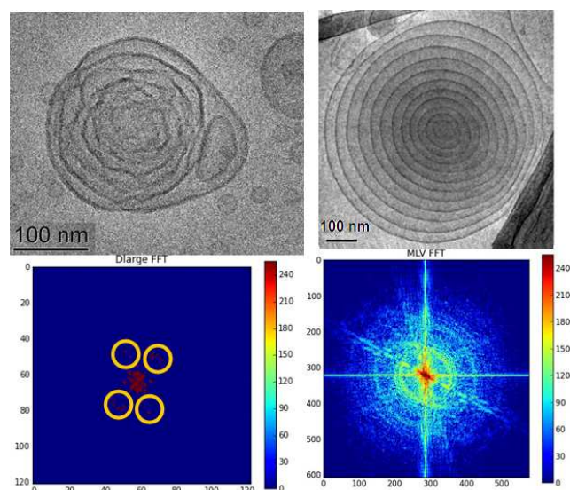
Figure 2. (Top) Cryo-TEM images presenting a topological comparison between a cubosome precursor particle with very large aqueous channels (left) and a multilamellar lipid vesicle (right). The scale bar in the images is 100 nm. (Bottom) Corresponding Fast Fourier Transformations (FFT) of the Cryo-TEM images with cubic lattice peaks on the left panel highlighted by yellow circles. The percentage of the cationic lipid is 15 mol.% (left panel) and 25 mol.% (right panel).
