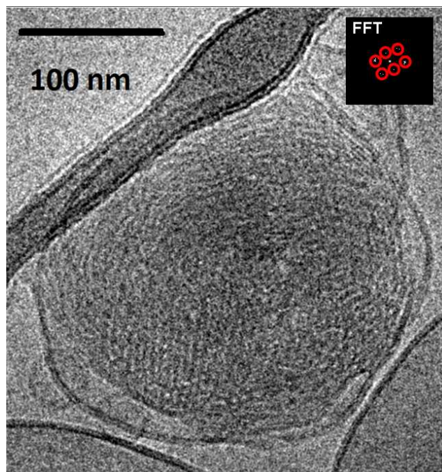
Figure 4. Cryo-TEM image demonstrating that the reduction of the interfacial charge (10 mol.% cationic lipid) may yield liquid crystalline nanoparticles of denser inner packing of the lipid membranes. Vesicular bilayer membranes are present in a coexistence with the cubosome lipid nanoparticles at ambient temperature. Depending on the orientation of the nanoparticles with respect to the electron beam, the nanochannel organization may not be laterally well visible.
