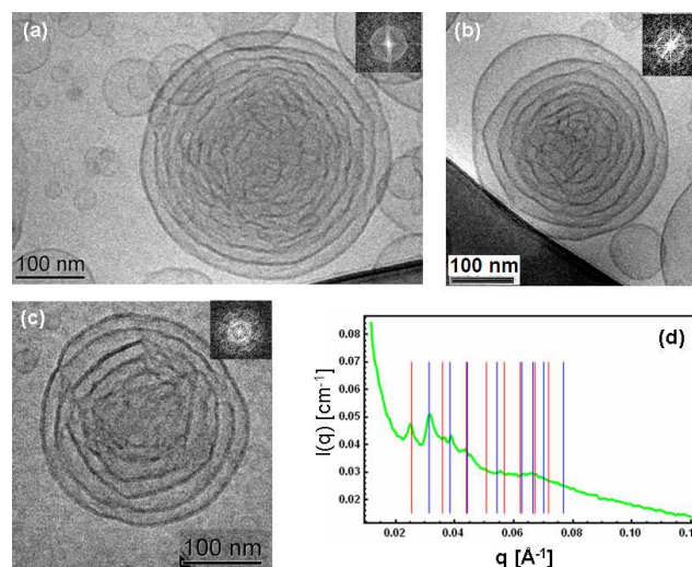
Figure 1. (a-c) Cryo-TEM images of cationic lipid cubosome intermediates with extra-large water channels (FFT are given as insets). (d) SAXS pattern of the same sample demonstrating the coexistence of Pn3m (double diamond) (blue bars representing the sequence \sqrt{2} : \sqrt{3} : \sqrt{4} : \sqrt{6} : \sqrt{8} : \sqrt{9} : \sqrt{10} of peaks positions) and Im3m (primitive) inner cubic lattice structures (red bars indicating the sequence \sqrt{2} : \sqrt{4} : \sqrt{6} : \sqrt{8} : \sqrt{10} : \sqrt{12} : \sqrt{14} : \sqrt{16} of peaks positions). The nanoparticle sample composition is derived from MO/DOMA/DOPE-PEG 2000 (82/15/3 mol%) LC membranes dispersed in excess buffer medium. The SAXS pattern (d) is representative for scattering from dispersed nanoobjects with internal liquid crystalline structure. It differs from a diffraction pattern of a bulk lipid mixture.
