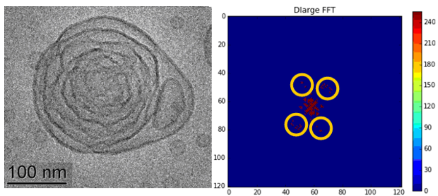
Liquid crystalline cationic cubosome nanoparticle with very large aqueous channels (cryoTEM image and the corresponding FFT pattern)
