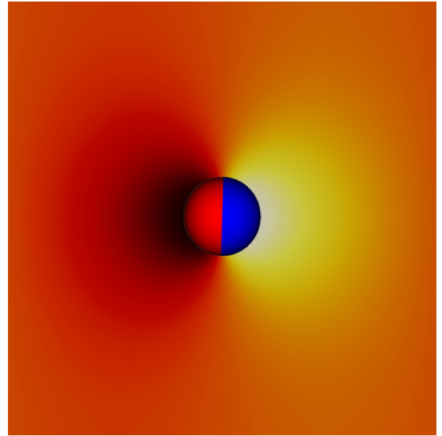
FIG. 7: Plot of the relative height of the interface. Influenced by a magnetic torque, the Janus particle reorients, leading to dipolar interface deformations: the interface is depressed on one side of particle (black) and raised on the other side (yellow). The interface is flat in the orange/red regions. These dipolar interface deformations are dynamically tunable, providing a route to generate tunable capillary-driven assembly at fluid interfaces.
