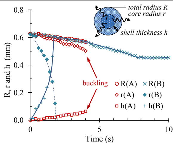
Fig. 4: Evolution of the total droplet radius R , core radius r and shell thickness h as functions of time. A (red dots) and B (blue dots) corresponds to droplets of
