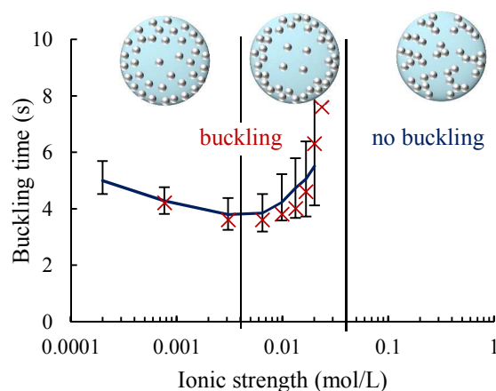
Fig. 5: Evolution of buckling time as a function of ionic strength. Red crosses correspond to experimental values whereas the blue curve corresponds to theoretical values computed from equation (12). Errors bars for experimental buckling times are too small to appear. Errors bars for calculated buckling times come from the measurement of zeta potential, input of equations (6) and (7).
