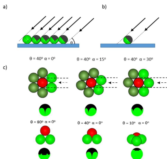
Figure 2 (a) Glancing angle evaporation onto a colloidal crystal modifies the cap shape as the glancing angle ( \theta ) is varied due to the potential for neighbouring colloids to shadow the line of sight path of the metal (black shading, arrows indicate direction of metal source). (b) If colloidal coverage is sufficiently sparse, changing the glancing angle, \theta , will not affect the deposited cap shape which will remain hemispherical. (c) Top section: At a fixed glancing angle, the orientation of the colloidal crystal ( \alpha ) relative to the metal source will produce variations in the deposited cap shape. The resulting deposited metal pattern on the red-sphere is shown below, light green spheres are responsible for the shadowing effects. Bottom section: The effect of varying glancing angle for a fixed crystal orientation is depicted. As the glancing angle is reduced, the patch coverage is reduced, and the perimeter shape is also altered.
