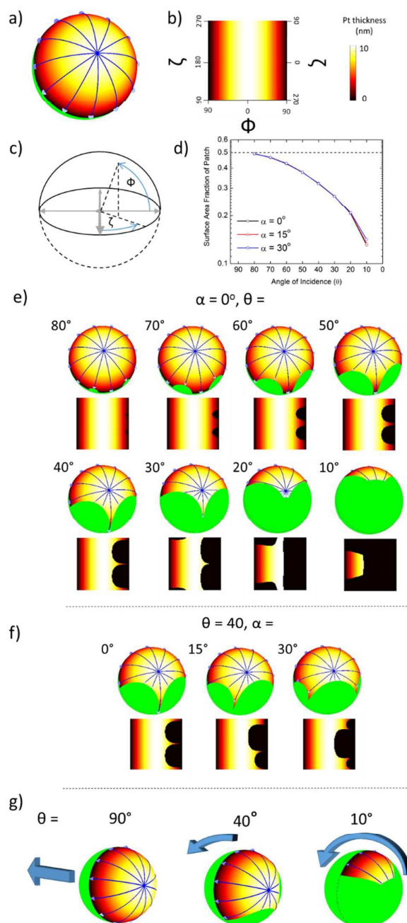
Figure 6 (a) 3D model of a Janus swimmer without shadowing. (b) Cap shape and thickness diagram represented in unwrapped 2D format using altitude and azimuthal coordinates and colour representation plot of platinum cap thickness from 0 to 10 nm. (c) Schematic representation of the altitude \Phi and azimuthal \zeta angles. (d) Graphical representation of overall patch area coverage with \theta for \alpha ( 0^\circ , 15^\circ and 30^\circ ). (e) 3d and 2d representation of the cap (same format as 6a,b) for \theta = 80^\circ to 10^\circ at \alpha = 0^\circ . (f). 3d and 2d representation of the cap (same format as 6a,b) for \alpha = 0^\circ , 15^\circ and 30^\circ at \theta = 40^\circ . (g) Schematic representation of changing cap shape
