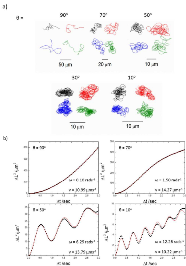
Figure 4. (a) Representative x y plot trajectories (30 seconds) for 1.9 μm diameter Janus colloids re-dispersed into 10 % H 2 O 2 solutions after platinum evaporation onto a colloidal crystal at a range of glancing angles. (b) Representative MSD plots from Δt 0.0 to 3.0 seconds for microsimmers prepared from colloidal crystals at 90°, 70°, 50° and 10° θ, a-d respectively. Black points represent experimental data and the red line is generated from equation 1 to find ω and v
