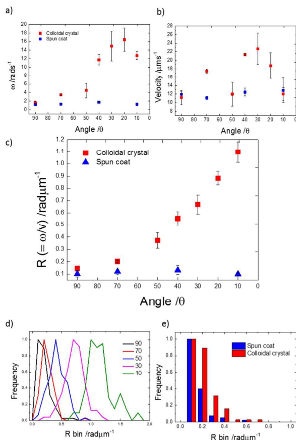
Figure 5 (a). Angular velocity ( \omega ) profile of microswimmers prepared from colloidal crystals (red) and sparsely spun coat colloids (blue) for a range of angles from 0 to 90° \theta . (b) Velocity ( v ) profile of microswimmers prepared from colloidal crystals (red) and sparsely spun coat colloids (blue) for a range of angles from 90° to 10° \theta . (c) Ratio ( R ) between \omega and v for microswimmers prepared from colloidal crystals (red) and sparsely spun coat colloids (blue) for a range of angles from 90° to 10° \theta . (d) R value distribution of microswimmers prepared from colloidal crystals for angles of 90° (black), 70° (Red), 50° (blue), 30° (pink) and 10° (green) \theta . (e) R value distribution for microswimmers prepared from spin coating (blue) and colloidal crystals (red) at 90° \theta
