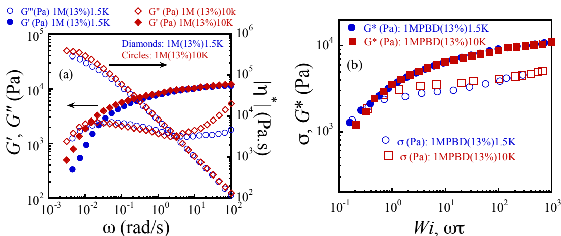
Fig. 3 (a): Small amplitude oscillatory shear (SAOS) measurement of two well-entangled PBD solutions. Dynamic storage, loss moduli and complex viscosity of 1M(13%)1.5K and 1M(13%)10K as a function of frequency using strain amplitude of 5% at room temperature (geometry: a 20 mm parallel-disk cell with separation of 1 mm). (b) Steady shear stress versus Wi (geometry: a 20 mm parallel disk with gap distance of ca. 50 \mu\text{m} ), along with the oscillatory shear data of G^* versus the dimensionless oscillation frequency ( \omega\tau ) for two PBD solutions.
