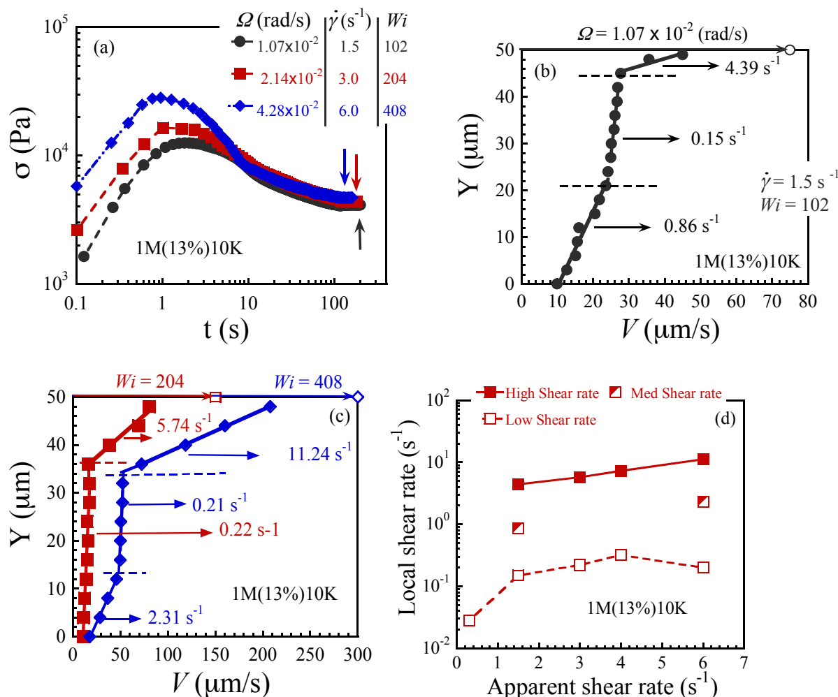
Fig. 8 (a) Shear stress response upon startup shear at different shear rates ( \dot{\gamma} : 1.5 , 3.0 and 6.0 \text{ s}^{-1} ) for 1M(13%)10K measured from the 20 mm-diameter parallel-disk shear cell with separation of 50 \mu\text{m} . (b) Shear banded velocity profile with formation of three flow regimes ( 0.15 , 0.86 and 4.39 \text{ s}^{-1} ) for apparent shear rate of 1.5 \text{ s}^{-1} in the steady state as indicated by the vertical arrow in (a). (c) Banded velocity profiles of 3.0 and 6.0 \text{ s}^{-1} in the steady state as indicated by the vertical arrow in (a). The rheometric velocities of upper plates are represented by open symbols in (b) and (c). (d) The local shear rates (obtained from PTV measurements) versus apparent shear rates for 1M(13%)10K.
