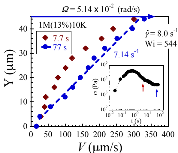
Fig. 12 Restoration of uniform velocity profile at high shear rate. Characterization of velocity profile at high shear rates = 8.0 \text{ s}^{-1} ( Wi = 544 ) at t = 7.7 and 77 \text{ s} . The inset shows a shear stress response upon startup shear at rate of 8.0 \text{ s}^{-1} .
