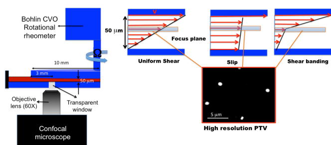
Fig. 2 (Left) Schematic illustration of rheo-confocal setup used for simultaneous rheometric and velocimetric measurements at room temperature with H = \text{ca. } 50 \mu\text{m} . (Right) Sketch of the parallel-disk geometry with three different velocity profiles: Uniform flow, slip and shear banding. The velocity profiles were measured by tracking the fluorescent melamine micro-beads with size of 1 \mu\text{m} .
