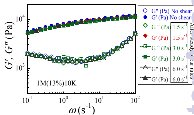
Fig. 11 Small amplitude oscillatory shear (SAOS) measurements before and after shear rates (with 650 s rest time for entanglement recovery after applying steady shear rates). Dynamic storage (closed symbols) and loss (open symbols) moduli of 1M(13%)10K as a function of frequency using strain amplitude of 5% at room temperature.
