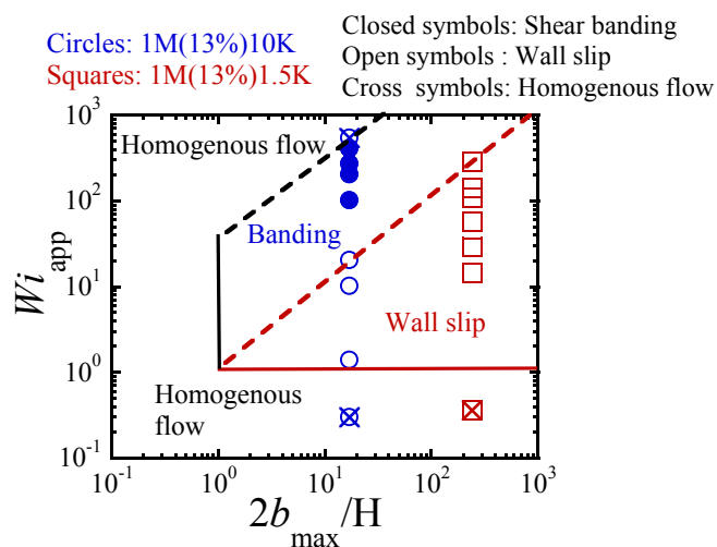
Fig. 13 Phase diagram in the parameter space of apparent Wi versus 2b_{\text{max}}/H for our findings at small gap for PBD solutions ( Z = 54 ) in different PBD solvents.
