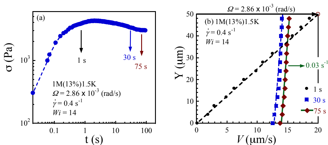
Fig. 5 (a) Shear stress response upon startup shear at rate of 0.4 \text{ s}^{-1} ( Wi = 14 ) for 1M(13%)1.5K. (b) The evolution of velocity profile at different times ( t = 1, 30 and 75 \text{ s} ). Velocity profile is linear across the gap, before stress maximum then massive slip developed at long times, in the 20 mm-diameter parallel-disk shear cell with separation of 50 \mu\text{m} . The open circle represents the velocity of upper plate, not PTV measurement.
