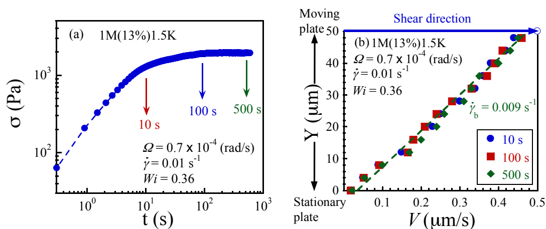
Fig. 4 (a) Shear stress response upon startup shear at rate of 0.01 \text{ s}^{-1} as function of time. The arrows indicate the moments when the velocity profiles were measured and presented in (b). Linear velocity profiles prevail at different times at such a low shear rate ( Wi = 0.36 ), involving the 20 mm-diameter parallel-disk with separation of 50 \mu\text{m} . The open circle represents the velocity of upper plate, not PTV measurement.
