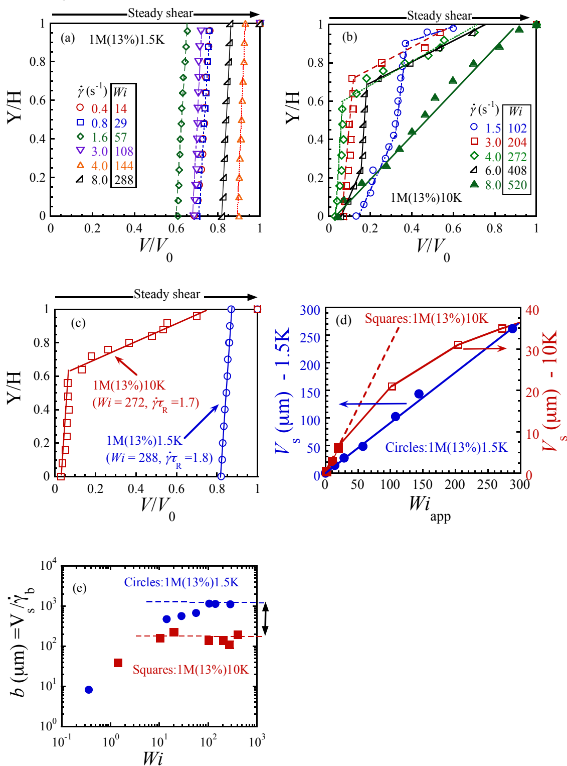
Fig. 9 Snap shots of velocity profiles in steady state for (a) 1M(13%)1.5K (slip-like behavior) and (b) 1M(13%)10K (bulk shear banding at 100 \leq Wi \leq 408 and uniform shear at Wi = 520 ). (c) The normalized velocity profiles for the two PBD solutions at the Wi = 288 and 272 ; \dot{\gamma}\tau_R = 1.8 and 1.7 , showing slip and shear banding respectively. (d) Slip velocity versus apparent Wi for the two PBD solutions where the vertical bar indicates the maximum difference. (e) Estimated slip length, b , versus apparent Wi for the two PBD solutions.
