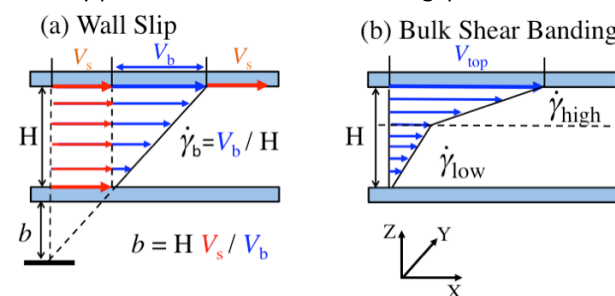
Fig. 1 Schematic diagram of the velocity profile within the gap of the shear geometry in presences of (left) wall slip, where b = V_s/\dot{\gamma}_b , and (right) bulk shear banding at the apparent shear rate.
