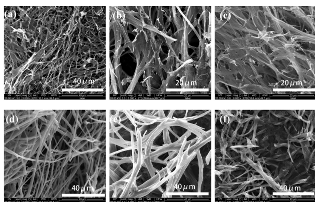
Fig. 2 SEM images of xerogels from Fe(III)-TPTA metallogels ( [\text{Fe}^{3+}] in mol/L, [\text{TPTA}] in g/L): a) 0.10 mol/L, 22.8 g/L; b) 0.15 mol/L, 33.7 g/L; c) 0.20 mol/L, 45.0 g/L; Fe(II)-TPTA metallogels ( [\text{Fe}^{2+}] in mol/L, [\text{TPTA}] in g/L) d) 0.010 mol/L, 4.4 g/L; e) 0.020 mol/L, 9.1 g/L; f) 0.030 mol/L, 14.4 g/L.
