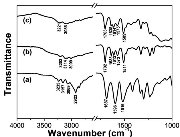
Fig. 5 FT-IR spectra of (a) crystal TPTA; (b) xerogel of Fe(III)-TPTA; (c) xerogel of Fe(II)-TPTA.
