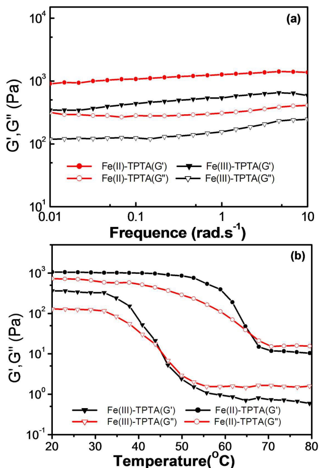
Fig. 4 Rheological properties of Fe(III)-TPTA gel (0.10 mol/L \text{Fe}^{3+} , 28.0 g/L TPTA) and Fe(II)-TPTA gel (0.010 mol/L \text{Fe}^{2+} , 6.0 g/L TPTA): (a) frequency sweep; (b) Temperature dependence of the storage shear moduli ( G' ) and the loss shear moduli ( G'' )
