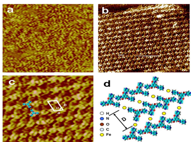
Fig. 8 (a) STM images of the assembling structure of TPTA on graphite surface with scan size ( 10.7 \text{ nm} \times 10.7 \text{ nm} , V = 640.0 \text{ mV} , I = 378.0 \text{ pA} ). (b) STM image of Fe(III)-TPTA self-assembled structure ( 18.3 \text{ nm} \times 18.3 \text{ nm} , V = 672.0 \text{ mV} , I = 376.0 \text{ pA} ). (c) Higher resolution STM image of Fe(III)-TPTA self-assembled structure ( 10.0 \text{ nm} \times 10.0 \text{ nm} ). (d) Proposed 2 dimensional molecular model for TPTA/ \text{Fe}^{3+} structures.
