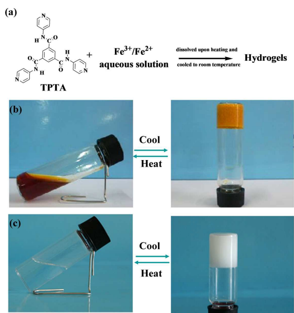
Fig. 1 (a) Metallo gels Formation; The photographs of gel-sol transition process of (b) Fe(III)-TPTA; (c) Fe(II)-TPTA
