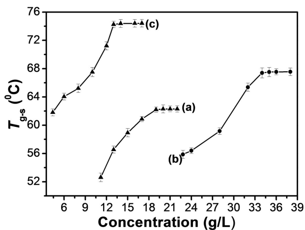
Fig. 3 Gel-sol transition temperatures ( T_{g-s} ) profiles of the metallogels prepared by varying concentrations of TPTA in aqueous solution containing: (a) 0.050 mol/L \text{Fe}^{3+} ; (b) 0.10 mol/L \text{Fe}^{3+} ; (c) 0.010 mol/L \text{Fe}^{2+} .
