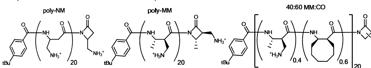
2 Figure 1. Chemical Structures of the nylon-3 polymers poly-NM, poly-MM and 40:60 MM:CO. All the polymers have an average chain length of approximately 20 subunits, and all are heterochiral.
