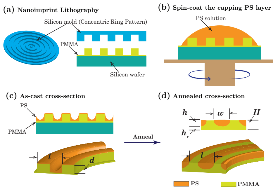
Figure 1. Schematics of the fabrication procedures for suspended PS rings: (a) Transfer concentric ring pattern from silicon mold to spin-cast PMMA film, via nanoimprint lithography; (b) Spin-cast PS on top of the PMMA pattern; (c) Cross-section of the as-cast bilayer film; (d) Cross-section of the film after annealing.
