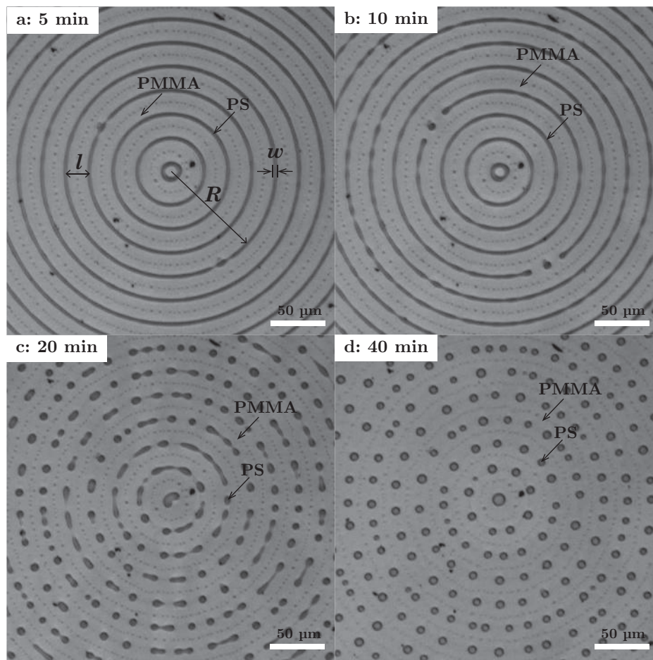
Figure 2. Optical image of concentric PS rings ( w = 3.1 \mu\text{m} , l = 20.2 \mu\text{m} , Sample A) annealed at 160 \text{ }^\circ\text{C} for the labeled duration: (a) newly formed, (b) undulation, (c) rupture and (d) shape relaxation of individual droplets.
