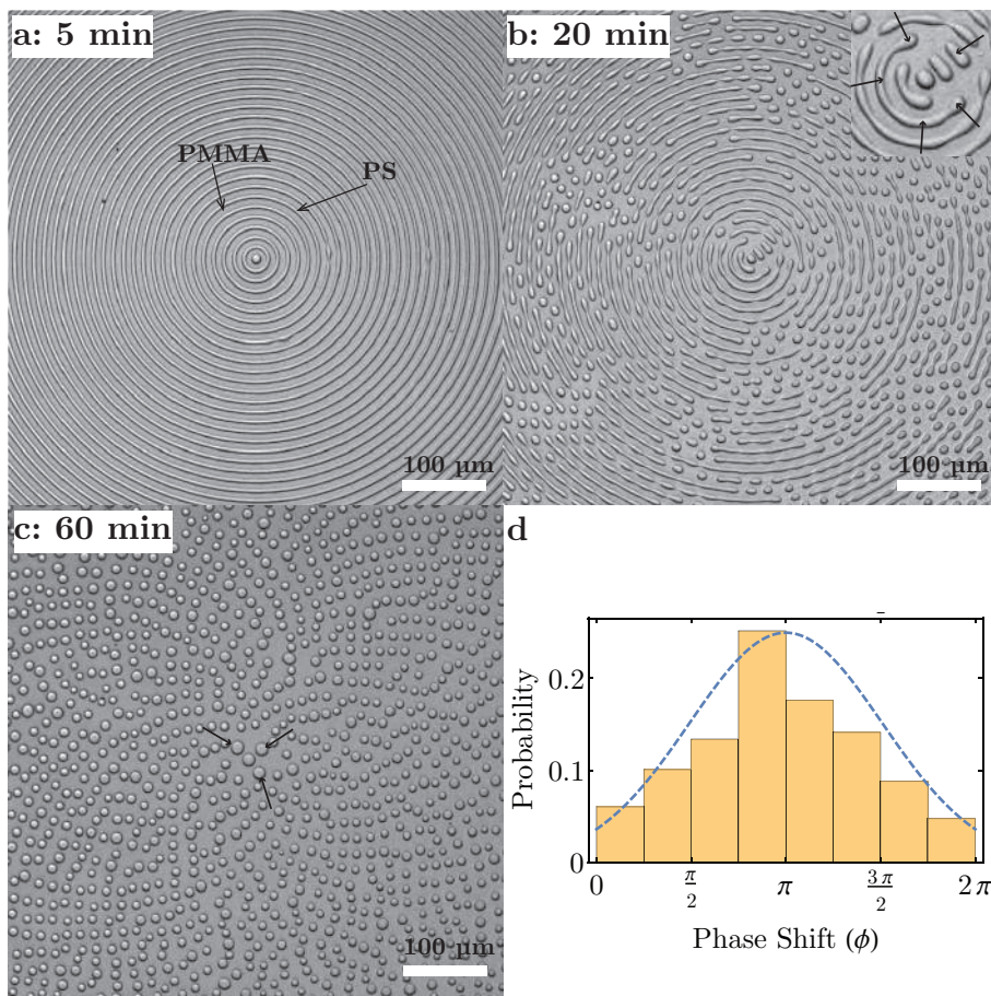
Figure 5. Optical images of Sample B annealed at 170 °C: (a) after leveling ( w = 4.6 \mu\text{m} , l = 12.1 \mu\text{m} ) and (b, c) rupture. (d) Distribution of \phi . The dotted line is a fit to a truncated normal distribution within domain [0, 2\pi) .
