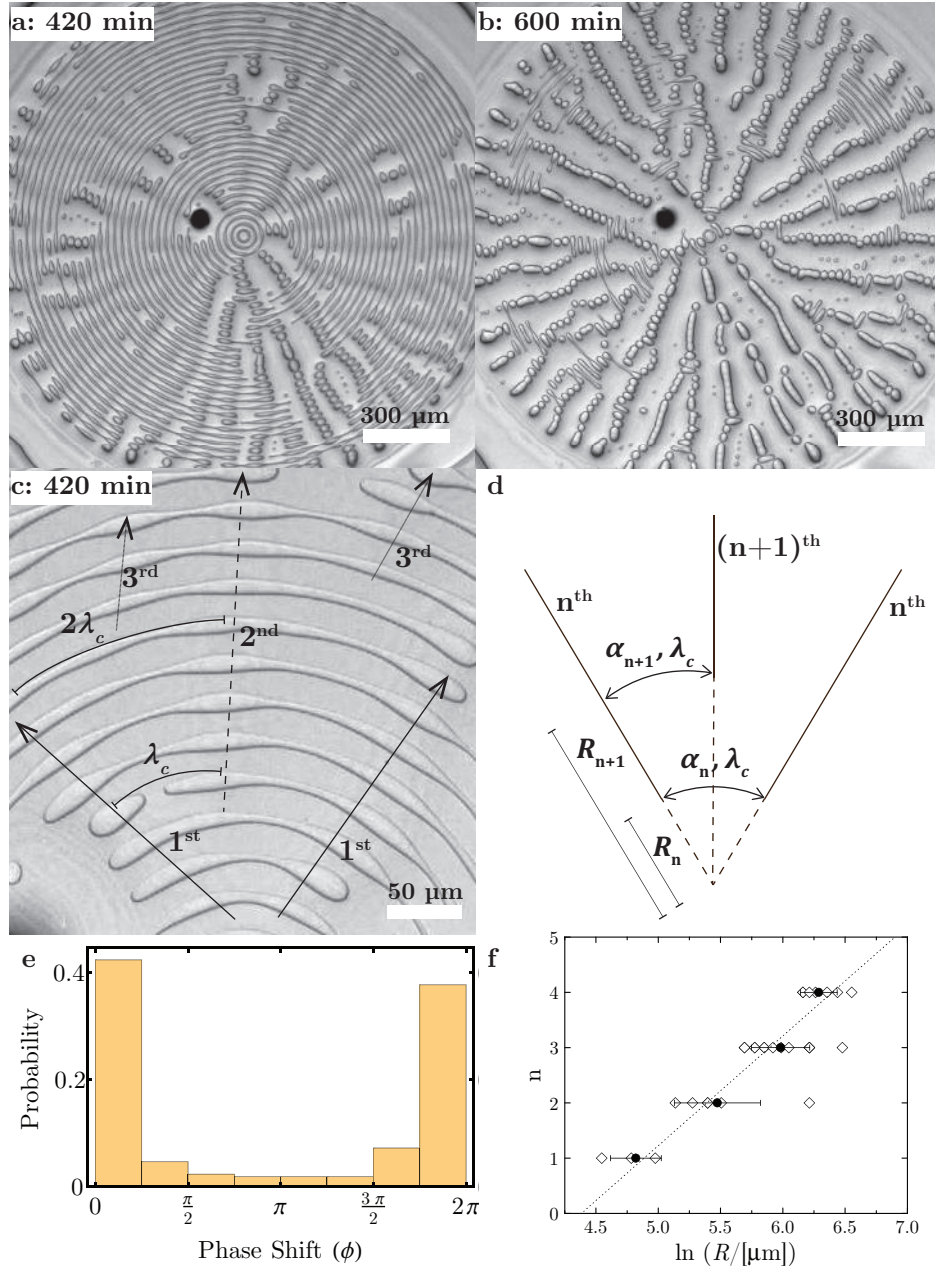
Figure 6. (a, b) Optical images of Sample C annealed at 170 °C for the labeled durations. Before undulation, w = 8.5 \mu\text{m} , l = 25.0 \mu\text{m} . (c) Close-up view of the undulation. (d) Schematic for the recursively “inserted” waves. (e) Distribution of \phi . The analysis was performed on the undulation stage (420 min). (f) Scaling between the order of generation n and R . Empty diamonds represent every new wave. The dotted line is a linear fit.
