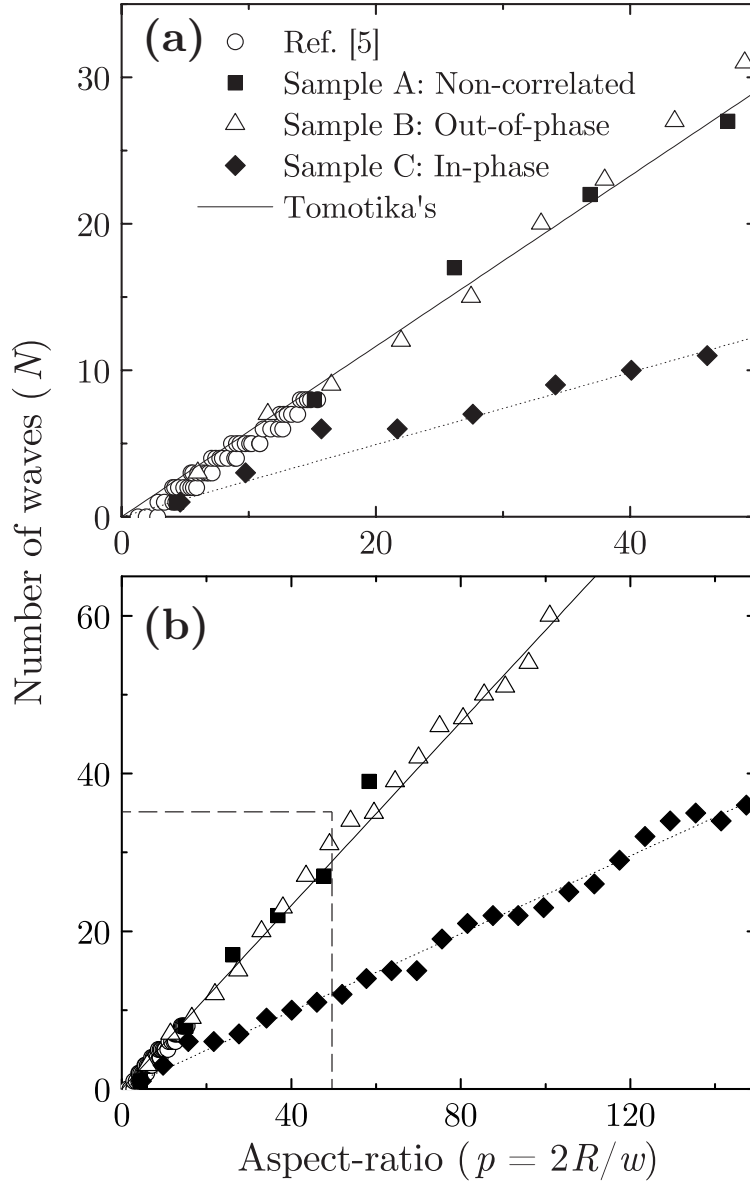
Figure 3. The number of capillary wavelengths plotted as a function of aspect ratio. The solid line is based on Tomotika’s theory. The dotted line is a linear fit to the “In-phase” data. The empty circles are adapted from reference [5]. (a) magnifies the dashed line region of (b) for improved readability, whereas (b) shows the full range of data.
