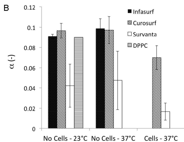
Fig. 6 Results of the drainage experiments. [A] The normalized height ( H ) as a function of rescaled time ( \tau ) for Survanta and Curosurf at 37 °C. The fit of Eq. 9 is shown as a dashed line and is used to obtain the fitting parameter \alpha . [B] The value for the fitting parameter \alpha for all lung surfactant replacements in the three studied conditions: at 23 °C without cells and at 37 °C with and without cells. The error bars correspond to the stochastic error of minimum 5 experiments.
