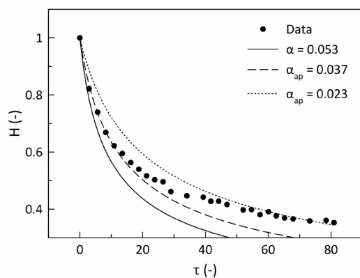
Fig. 10 Experimental results of the normalized height ( H ) as a function of rescaled time ( \tau ) for a Survanta film flowing over a cell covered geometry at 37°C. The rate of drainage, expressed by the fitting parameter \alpha_{ap} , decreases in time due to the portion of flow in the rough layer which becomes more important for thin films.
