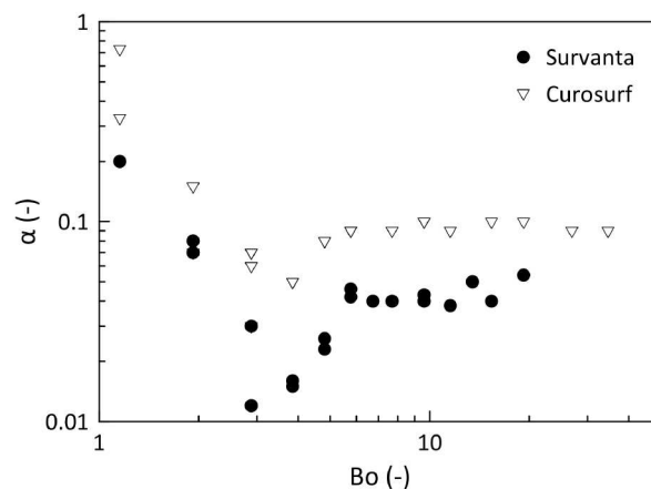
Fig. 5 The drainage rate characterised by the parameter \alpha for Curosurf, Survanta at room temperature, for different Bond numbers defined as the ratio of hydrostatic pressure ( P_H ) and capillary pressure ( P_C ).
