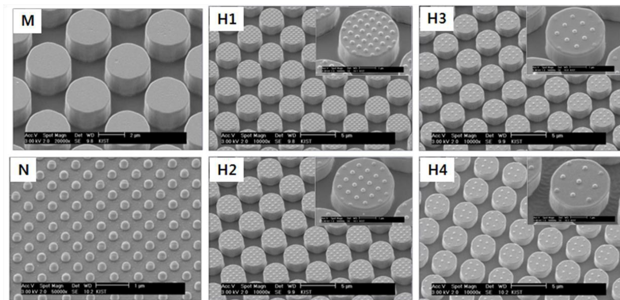
Fig. 1 Scanning electron micrographs of the fabricated patterns: M-micro, N-nano, H1-hierarchical pattern with 500-nm pitch nano-pillars; H2- hierarchical pattern with 625-nm pitch nano-pillars; H3- hierarchical pattern with 750-nm pitch nano-pillars; H4- hierarchical pattern with 1000-nm pitch nano-pillars.
