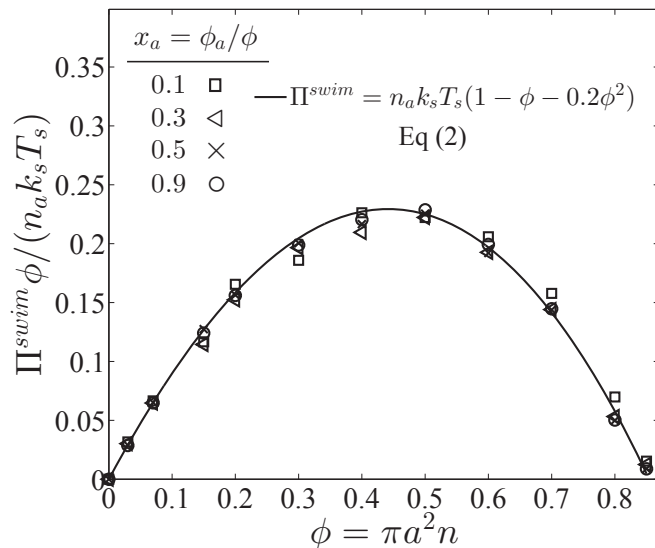
Fig. 3 Swim pressure exerted by active swimmers in a mixture as a function of the total area fraction \phi = \phi_a + \phi_d for different values of active composition x_a = \phi_a / \phi and fixed Pe_R \equiv a / (U_0 \tau_R) = 0.1 . Subscripts ‘a’ and ‘d’ refer to active and passive particles, respectively. The solid curve is the mechanical theory Eq 2 and the symbols are BD simulations. The swimmer activity k_s T_s \equiv \zeta U_0^2 \tau_R / 2 .
