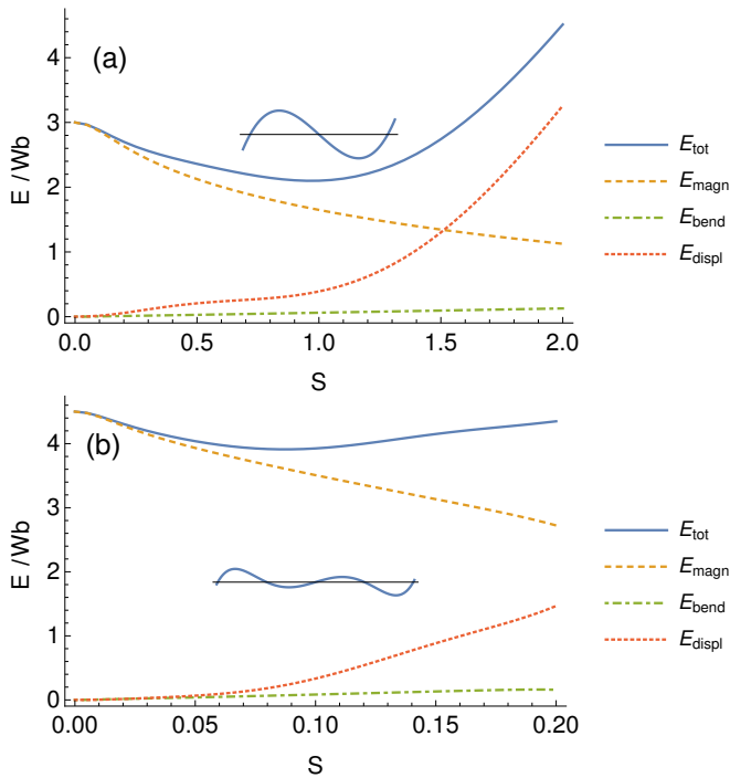
Fig. 6 Contributions to the total energy as a function of the amount S of deformation and minimized with respect to x_1 and x_2 for a chain of the shape given by Eq. (5). Here we show the cases (a) M = 2 , L = 3b and (b) M = 4 , L = 4.5b . The total energy E_{tot} has a global minimum as a function of S , which corresponds to the most stable chain shape. We always observed the global minimum for symmetric shapes.
